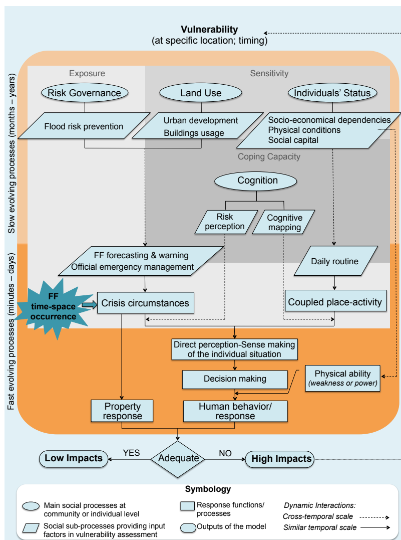
Figure 1 Conceptual model of dynamic vulnerability drivers leading to flash flood impacts. Source: Terti et al. (2015).
