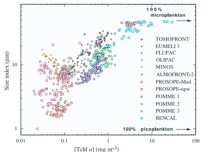
Figure 5. Variations of the size index, estimated using equation (2), as a function of the \text{Tchl } a concentration.
