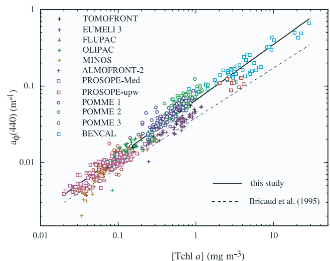
Figure 2a. Variations of the absorption coefficients of phytoplankton at 440 nm as a function of the Tchl a concentration, for the various cruises (see Table 1). Only samples collected within the first optical depth have been considered in these figures and all following ones. The regression line (equation (5)) is shown as a solid line. The relationship obtained by Bricaud et al. [1995] (equation (5')) is shown for comparison as a dashed line.
