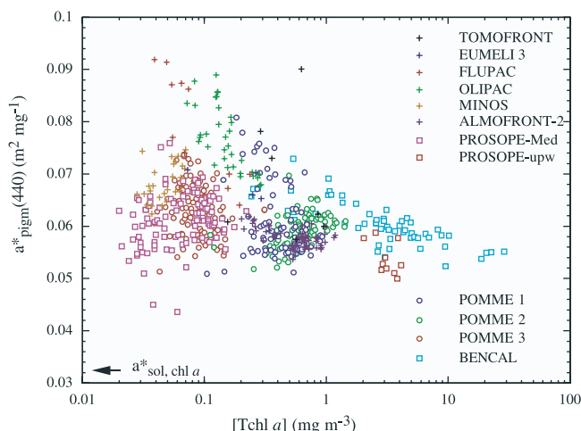
Figure 6. Variations of the chl-specific absorption coefficient of pigments at 440 nm, a_{\text{pigm}}^*(440) (obtained by using equation (4'') and then normalizing by the Tchl a concentration), as a function of the Tchl a concentration.
