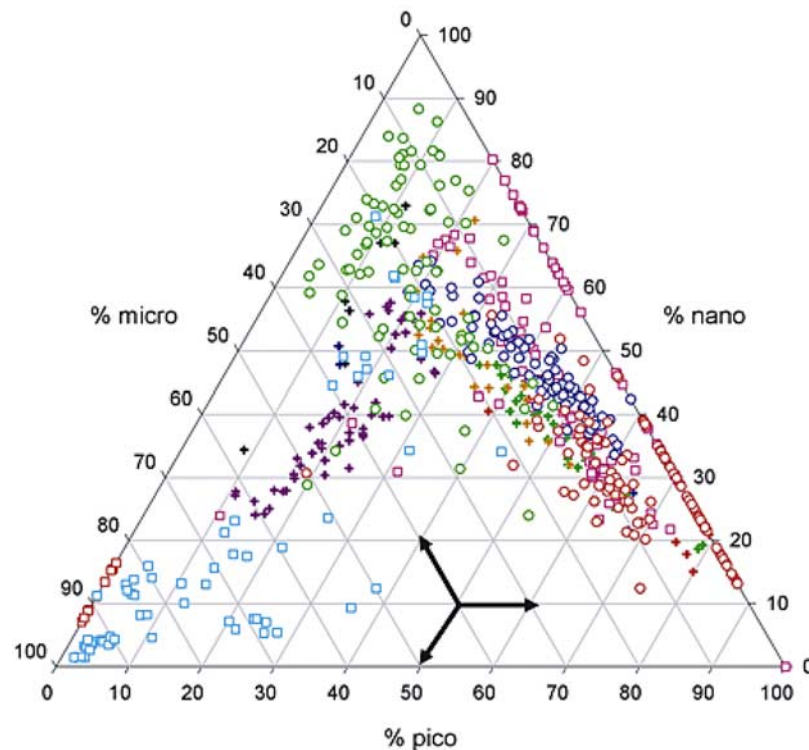
Figure 4. Ternary plot showing the relative contributions (percent) of picophytoplankton, nanophytoplankton, and microphytoplankton to total biomass, estimated from the relative concentrations of some taxonomic pigments (equations (1a)–(1c)). The symbols are as in Figure 3. For each sample the relative contribution of a size class to total biomass can be read on the corresponding axis as indicated.
