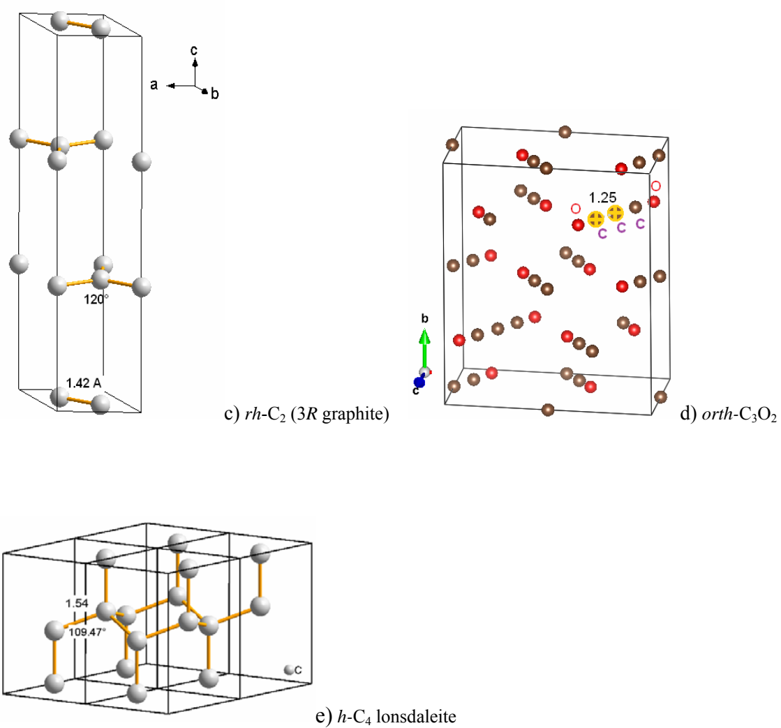
Fig. 1. Sketches of the structures a) rh\text{-NaN}_3 , b) h\text{-B}_{36}\text{C}_9 , c) rh\text{-C}_2 (3R graphite), d) orth\text{-C}_3\text{O}_2 , and e) h\text{-C}_4 lonsdaleite in a 2\times 2\times 1 supercell (rhombohedral structures are represented in hexagonal settings). Remarkable interatomic distances and angles are displayed in Å and deg ( ^\circ ), respectively.
