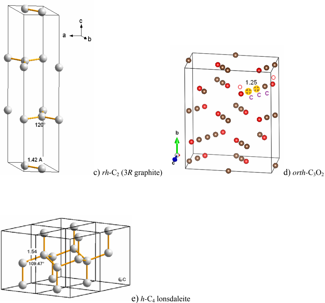
Fig. 1. Sketches of the structures a) rh-NaN_3 , b) h-B_{36}C_9 , c) rh-C_2 (3R graphite), d) orth-C_3O_2 , and e) h-C_4 lonsdaleite in a 2 \times 2 \times 1 supercell (rhombohedral structures are represented in hexagonal settings). Remarkable interatomic distances and angles are displayed in Å and deg ( ^\circ ), respectively.
