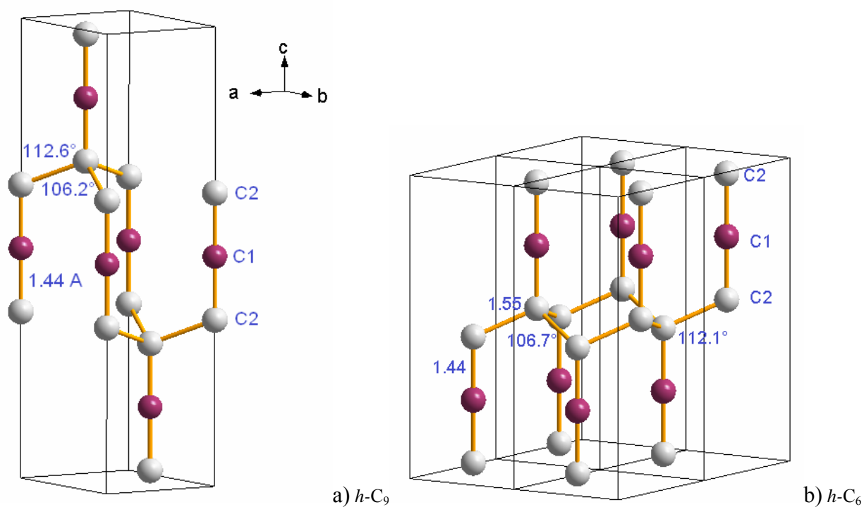
Fig. 2. Sketches of the new tricarbon rhombohedral based structures represented in hexagonal settings. a) rh-C_3 ( h-C_9 ) and b) h-C_6 derived from C_4 lonsdaleite (cf. Fig. 1d) shown in a 2 \times 2 \times 1 supercell. Remarkable interatomic distances and angles are displayed in Å and deg ( ^\circ ), respectively.
