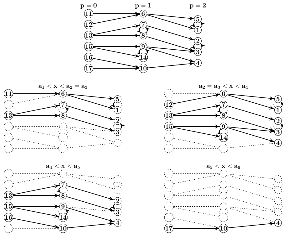
Figure 6: Top: the complete graph containing all the auxiliary functions obtained via the construction presented in Section 3.3 in the case of the example of Figure 5. Bottom: The actual evaluation graph obtained when computing the value of the spline functions at different locations x .
