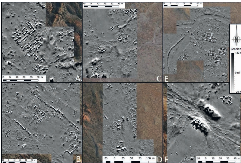
Figure 2. Magnetic maps around urban structures at the site of Larsa (Darras, 2019).
