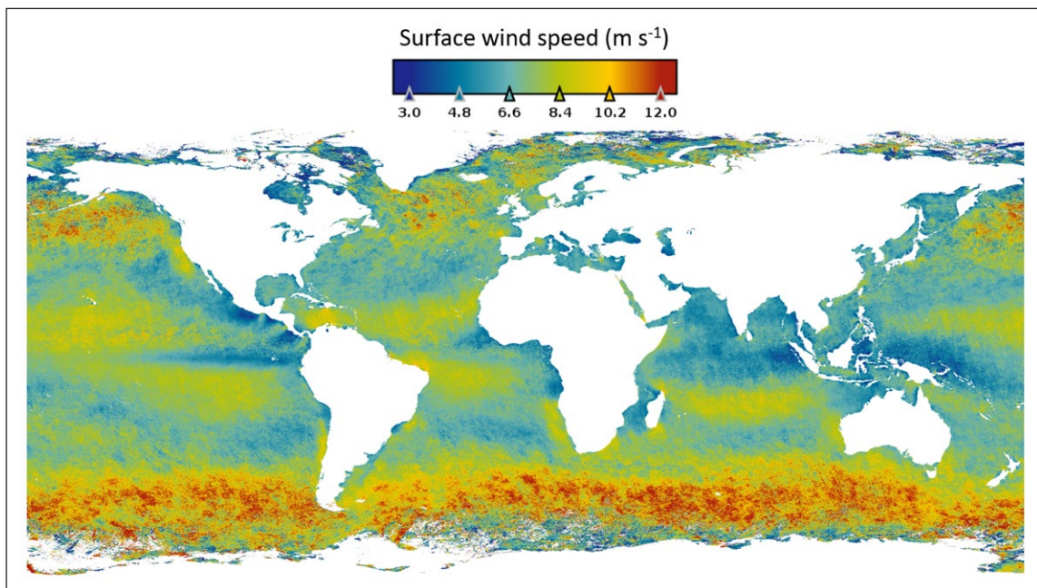
Figure 12: Global wind speed fields derived from the sun-glitter signal. Annual average of the sea surface wind speed for 2007 obtained from inversion of the sun-glitter signal measured by PARASOL for clear sky conditions (data available from ICARE/CNES). DOI: https://doi.org/10.1525/elementa.331.f12
