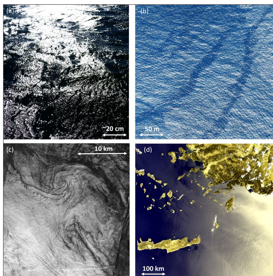
Figure 11: Examples of sun-glint patterns at different spatial scales. (a) Image of the sea surface under gust wind conditions taken from a reflex digital camera. (b) Aerial photography of sea surface with visible surfactant filaments. (c) Sentinel-2A image (4 July 2015) in the 2190-nm channel where sun glint is the most intense signal over water; the sun-glitter patterns highlight some geophysical phenomena such as eddies, ship wakes, and wave packets; (d) Sentinel-3 RGB image (10 May 2016) over the eastern Mediterranean Sea; high sun glint is readily visible on the right side of the image. DOI: https://doi.org/10.1525/elementa.331.f11
