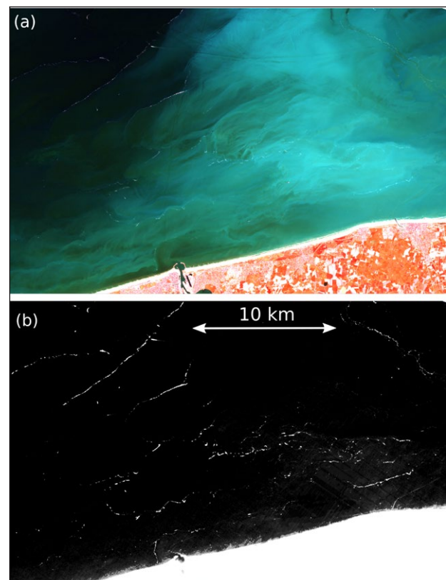
Figure 2: Fine-scale features of a coastal phytoplankton bloom. (a) Sentinel 2A/MSI RGB composite of the Belgian coastal zone on 1 May 2016 (10:53UTC) indicating fine-scale features in ocean colour satellite imagery, such as foam produced by Phaeocystis globosa , and (b) near infrared image of the same scene. Satellite image suggested by Q. Vanhellemont. DOI: https://doi.org/10.1525/elementa.331.f2
