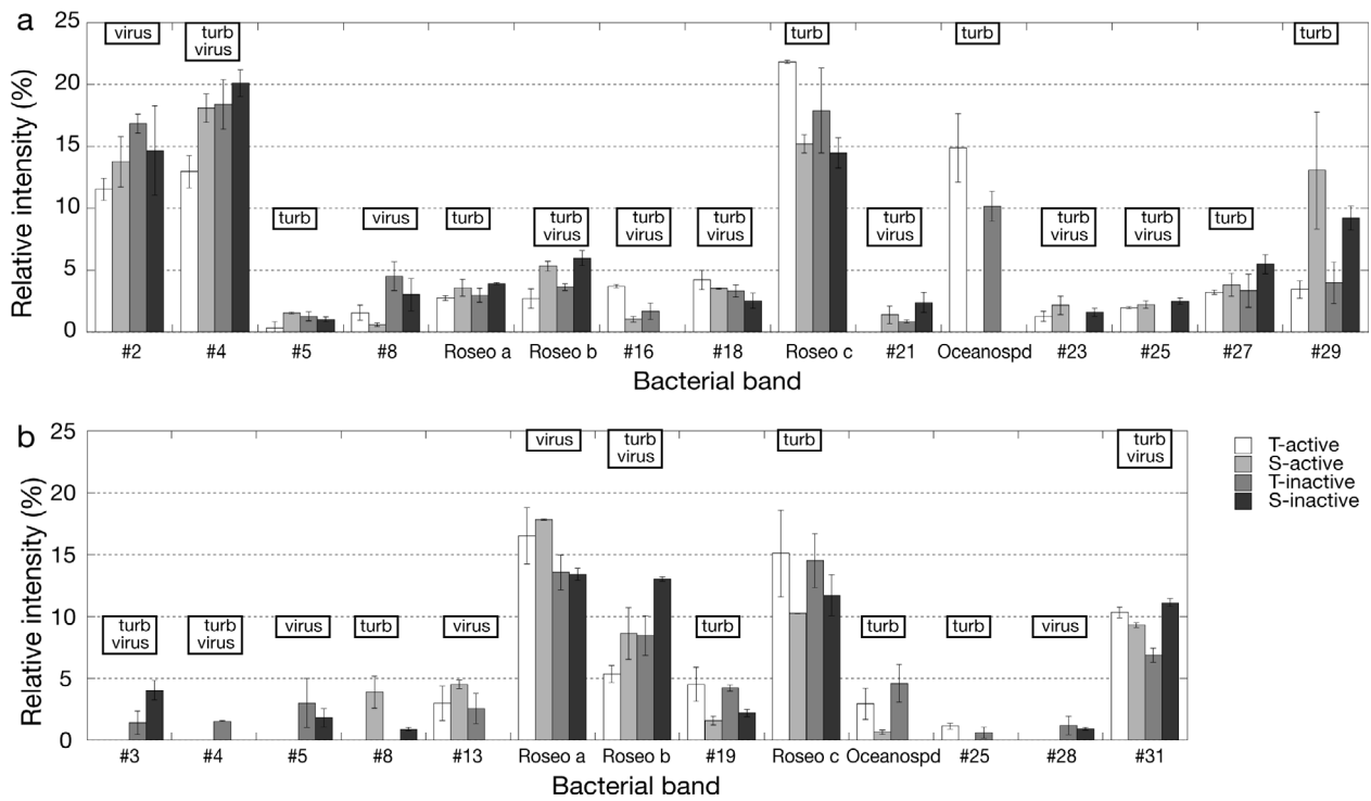
Fig. 5. Relative band intensities of all bacterial bands from the final assemblage in (a) TV 1 and (b) TV 2 that were influenced significantly by viruses and/or turbulence. Values are means ± SD, n = 3. The experimental factor(s) [virus and turbulence (turb)], are indicated above the columns. Treatment labels as in Fig. 3
