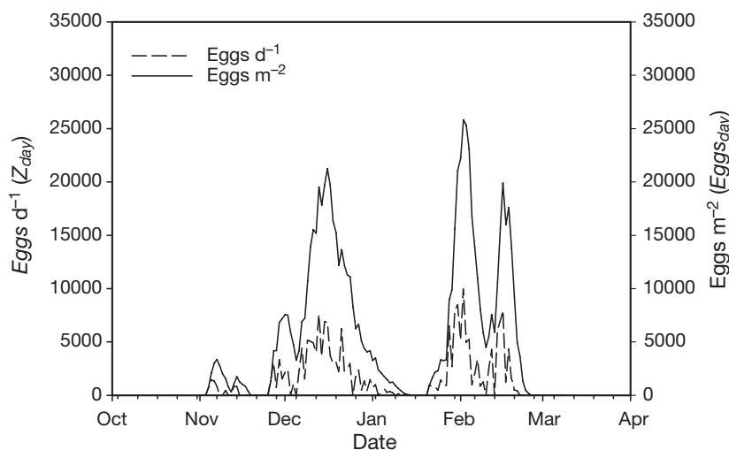
Fig. 5. Euphausia superba . Predicted concentration of eggs released by the krill population ( Z_{\text{day}} , dashed line) and the concentration residing in the water column ( Eggs_{\text{day}} , solid line) on each day of the productive season
