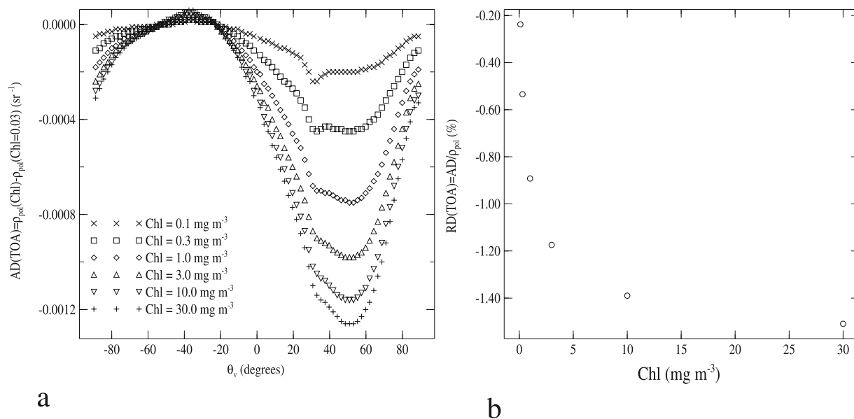
Figure 4. (a) Absolute difference AD between \rho_{pol}(\text{TOA}) at a given value of Chl and \rho_{pol}(\text{TOA}) at the reference value of Chl = 0.03 \text{ mg m}^{-3} (see equation (10)) at 443 nm. The conditions of simulation are already mentioned in Figure 1. (b) Relative difference RD = AD/\rho_{pol} (in %) between the polarized reflectance at a given value of Chl (corresponding to the x -axis) and a reference value of Chl (i.e., Chl_{ref} = 0.03 \text{ mg m}^{-3} ). The calculation is carried out at 443 nm, at the Brewster viewing angle (i.e., \theta_v = +54^\circ ) and at \text{TOA} .
