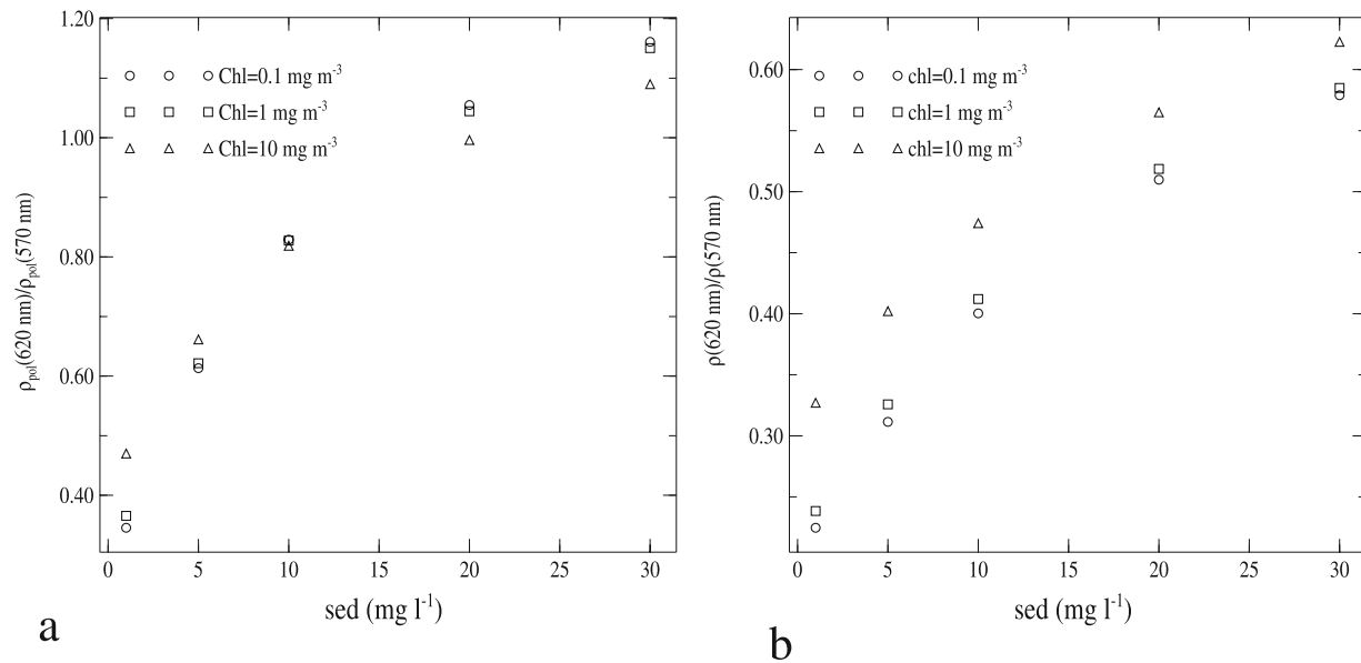
Figure 13. (a) Spectral ratio \rho_{pol}(620 \text{ nm})/\rho_{pol}(570 \text{ nm}) as a function of sed . The calculation is made at 0^\circ , \theta = 100^\circ and for different values of Chl (i.e., Chl = 0.1, 1 and 10 \text{ mg m}^{-3} ). (b) Similar as Figure 13a except the spectral ratio of the total reflectance \rho(620 \text{ nm})/\rho(570 \text{ nm}) is plotted.
