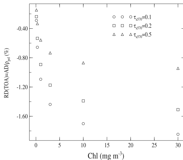
Figure 5. Relative difference RD = AD/\rho_{pol} (in %) between the polarized reflectance at a given value of Chl (corresponding to the x -axis) and a reference value of Chl (i.e., Chl_{ref} = 0.03 \text{ mg m}^{-3} ) for different values of the aerosol optical depth \tau_a at 570 nm. The calculation is carried out at 443 nm, at the Brewster viewing angle (i.e., \theta_v = +54^\circ ) and at \text{TOA} .
