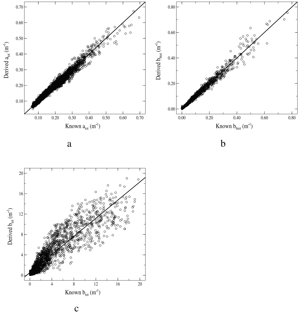
Figure 3. Comparison between the retrieved and the known IOP at 555 nm: (a) a_{\text{tot}} , (b) b_{\text{btots}} , and (c) b_{\text{tot}} . The nadir-viewed subsurface remote sensing reflectance spectra were inverted (case S, see text).
