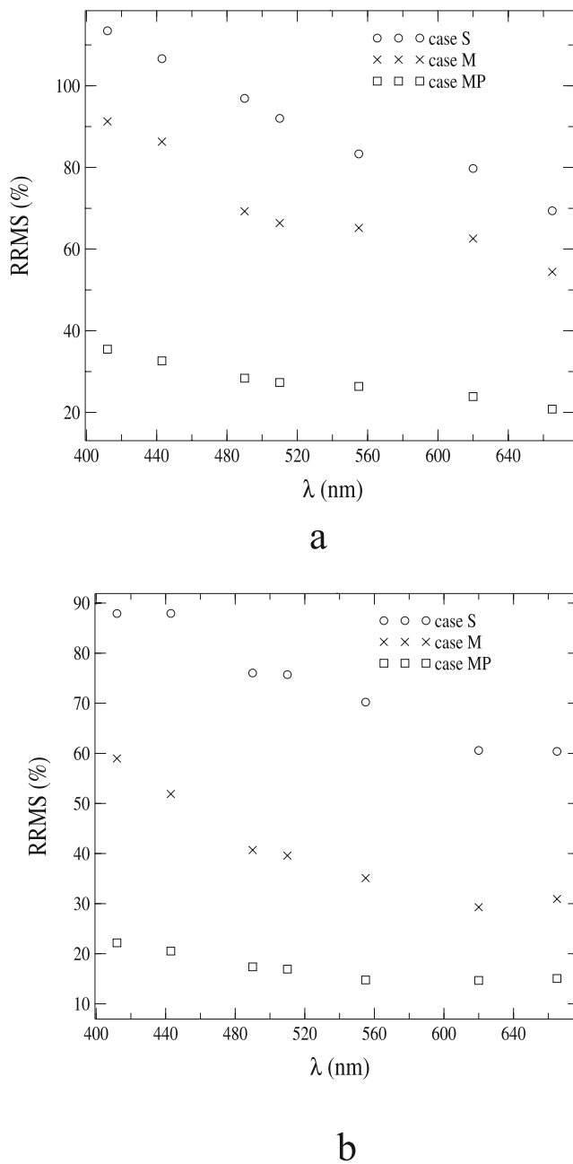
Figure 7. Spectral variation of the RRMS (in %) obtained for the retrieval of (a) b_{ph} and (b) b_{NC} . Cases S, M, and MP are reported.
