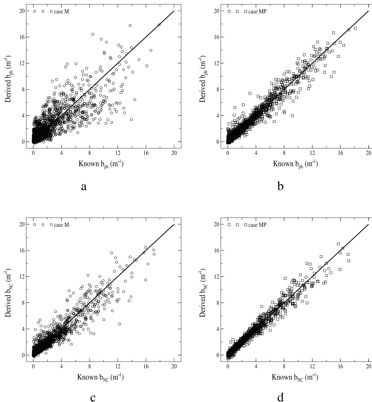
Figure 8. Same as Figure 5 but for the retrieval of the following scattering coefficients: (a) b_{\text{ph}} : case M, (b) b_{\text{ph}} : case MP, (c) b_{\text{NC}} : case M, and (d) b_{\text{NC}} : case MP.
