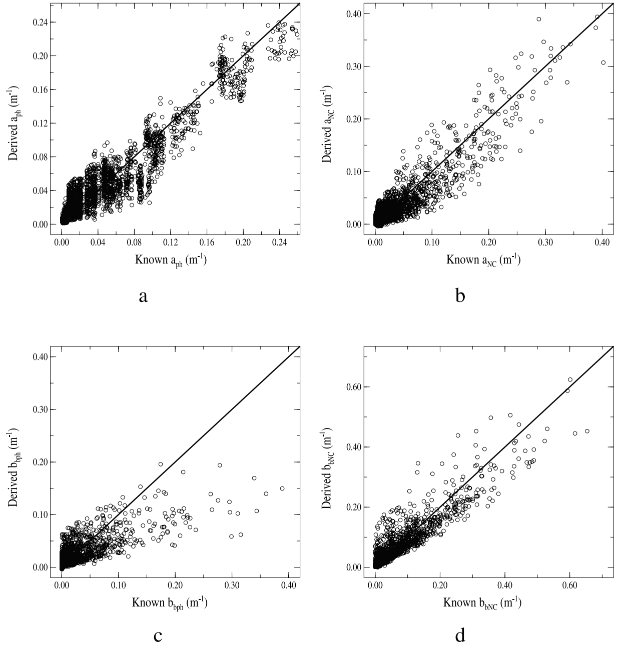
Figure 4. Same as Figure 3 but for the retrieval of the following IOP: (a) a_{\text{ph}} , (b) a_{\text{NC}} , (c) b_{\text{bph}} , and (d) b_{\text{bNC}} .
