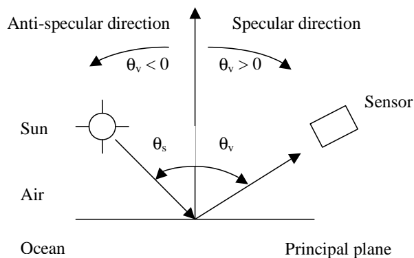
Fig. 1. Geometry of observation of the REFPOL instrument in the principal plane.
