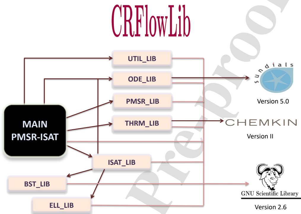
Figure 1: Schematic representation of PMSR-ISAT main program and CRFlowLib libraries, with an indication of their internal and external dependencies.
