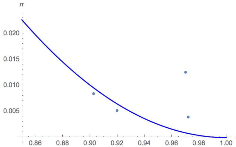
Figure A.2 Fitting the function \pi(\cdot) for the four European countries (Sweden included): \gamma^{\text{EUR}} = 1.995 .
