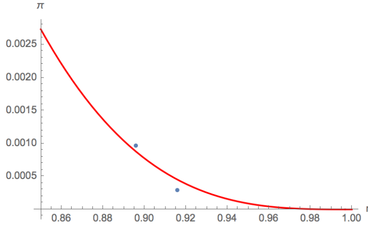
Figure A.1 Fitting the function \pi(\cdot) for the US and Canada: \gamma^{\text{NA}} = 3.110 .
