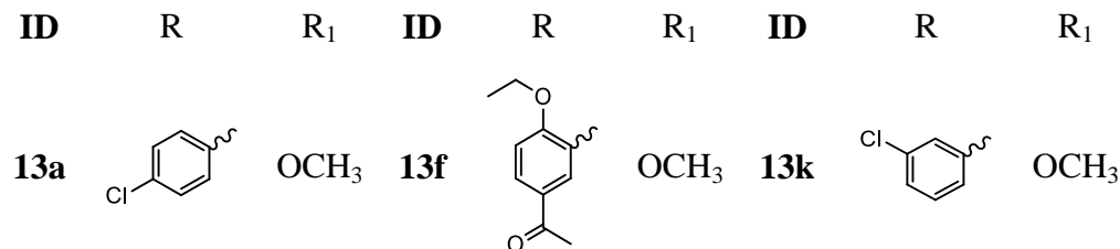
Scheme 3: Reagents and conditions: (a) i) oxalyl chloride, cat. DMF, dichloromethane, ii) DIPEA, dichloromethane; (b) i) aqu. NaOH, Methanol, reflux, ii) dil. HCl; (c) i) PyBOP, DIPEA, \text{H}_2\text{NOTHP} , THF, ii) dil. HCl, THF.
