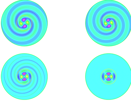
Figure 3: We represent the scattered fields for the same scattering experiment as in Figure 2 with an incident field being a Herglotz wave function with kernel g(\theta) = \exp(-2i\theta) but for different wave numbers. From top to bottom and left to right k = 6 , k = 6.5 , k = 7 , k = 7.223 (a transmission eigenvalue).
