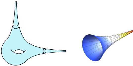
Figure 4: Sketch of a hyperbolic surface with 2 cusps (left) and part of a hyperbolic cusp (right) isometrically embedded into \mathbb{R}^3 .
