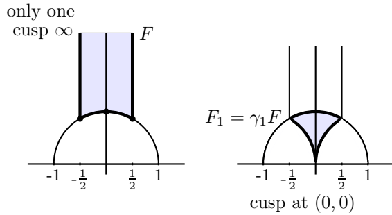
Figure 5: Left: Shaded region depicts the Ford fundamental domain F for \Gamma = SL_2(\mathbb{Z}) . Right: Shaded region depicts an equivalent fundamental domain F_1 = \gamma_1 F , where \gamma_1 : z \rightarrow -1/z . The image of F under \Gamma tessellates \mathbb{H} .
