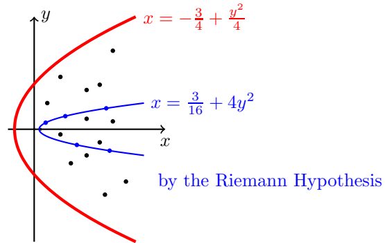
Figure 6: Black dots indicate possible location of transmission eigenvalues. There are infinitely many transmission eigenvalues on the inner parabola and all eigenvalues lie inside the outer parabola. If the Riemann Hypothesis is true, all transmission eigenvalues lie on the inner parabola. There are no real transmission eigenvalues except for the trivial ones, at 0 and 1/4 .
