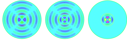
Figure 2: Illustration of a transmission eigenvalue for a dielectric medium formed by two concentric circles with outer radius = 1 and inner radius = 0.3. The refractive index n = 2 in the annulus and n = 3 in the inner circle. The wave number is k = 7.223 . Left: Incident field; a Herglotz wave function with kernel g(\theta) = \exp(-2i\theta) . Middle: Total field. Right: Scattered field (=0 outside the circle of radius 1).
