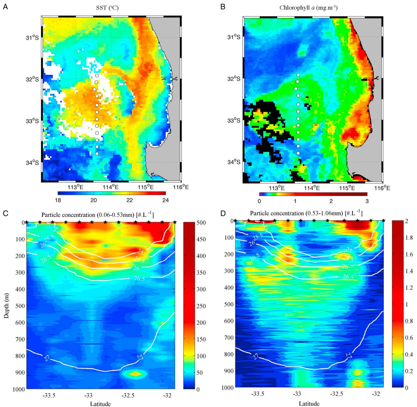
Figure 1. (a) Sea-surface temperature ( ^{\circ}\text{C} ) and (b) chlorophyll a ( \text{mg m}^{-3} ) derived from Moderate Resolution Imaging Spectroradiometer (MODIS) satellite, showing the mesoscale eddy in the Leeuwin Current (LC) off Australia. White circles indicate stations sampled. Spatial distributions of particles across the eddy: (c) Small (0.06–0.5 mm) and (d) large (0.5–1 mm) particles as measured by the Underwater Vision Profiler (UVP) shown in color, with isopycnals contoured in white.
