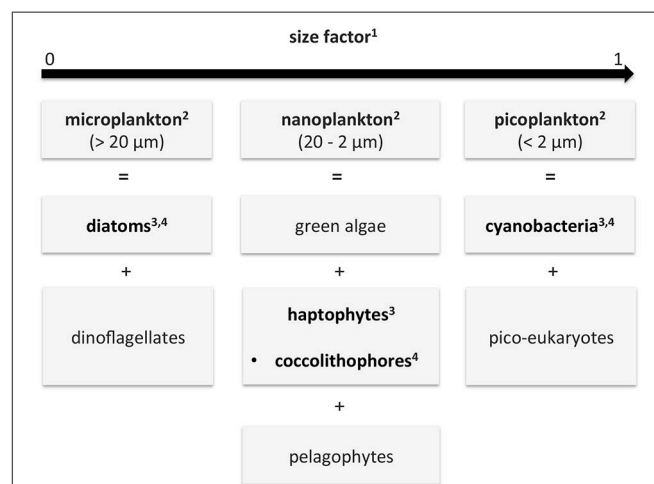
FIGURE 1 | Diagram describing the different phytoplankton classifications given by the different data products of this study and how they relate to each other: functional types (PFTs), size classes (PSCs) and size factor (Sf). In bold are the data used in this study: in the SynSenPFT algorithm (PFTs) and for validation (PSC and Sf). The numbers in the boxes indicate the corresponding references of the products used in this study: 1 Ciotti and Bricaud (2006), 2 Brewin et al. (2010, 2015), 3 Hirata et al. (2011), 4 Bracher et al. (2009) and Sadeghi et al. (2012). Note that different PFTs can vary among size classes, e.g., diatoms also can spread into the nanoplankton fraction.
