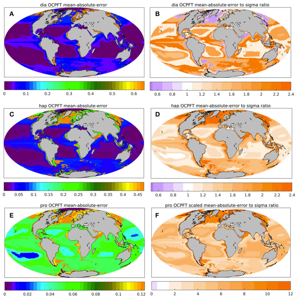
FIGURE 5 | Additional statistics assessing OC-PFT against in situ on the biomes grid by Hardman-Mountford et al. (2008): the mean-absolute-error (MAE, mgChla m^{-3} , A,C,E ) and the ratio of MAE to the OC-PFT unscaled uncertainties obtained based on the TC analysis ( B,D,F ) for diatom ( A,B ), haptophytes ( C,D ) and prokaryotes ( E,F ).
