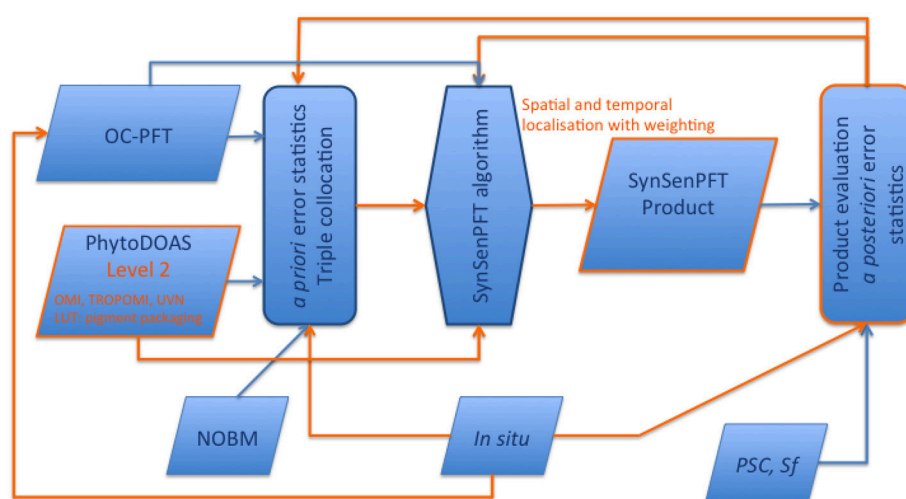
FIGURE 13 | Schematic presentation of the SynSenPFT system and development flowchart. In orange color possibilities for further improvements and/or augments are emphasized.
