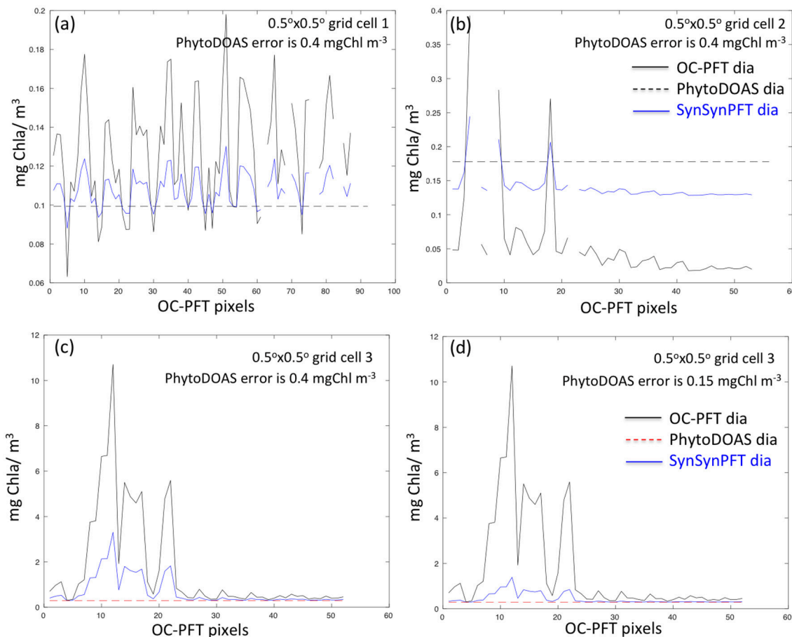
FIGURE 3 | Examples illustrating variability of OC-PFT and updated (nudged toward PhytoDOAS) SynSenPFT diatom Chla within three PhytoDOAS pixels with different OC-PFT Chla variability, PhytoDOAS Chla on average either lower (a,c) or higher (b) than OC-PFT Chla and given PhytoDOAS error statistics ( 0.4 \text{ mgChl m}^{-3} for a–c ). (c,d) depict SynSenPFT diatom Chla obtained for the same PhytoDOAS grid cell but assuming different PhytoDOAS errors: 0.4 \text{ mgChl m}^{-3} (c) and 0.15 \text{ mgChl m}^{-3} (d) . Thus, lower panels illustrate the sensitivity of SynSenPFT diatom Chla product to the assumed PhytoDOAS error statistics.
