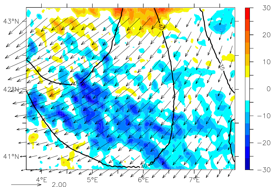
Figure 4. Same as Figure 3 for the horizontal Ekman advection of temperature (shades, units 10^{-8} \text{ }^{\circ}\text{C s}^{-1} ), Ekman transport (arrows, units \text{m}^2 \text{ s}^{-1} and scale in the lower left corner) every 10 grid points and Ekman layer depth (contours, units m).
