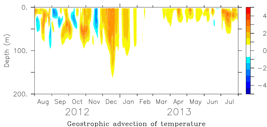
Figure 5. Temporal evolution of the domain average geostrophic advection of temperature ( 10^{-7} \text{ } ^\circ\text{C s}^{-1} ) as a function of depth (m).
