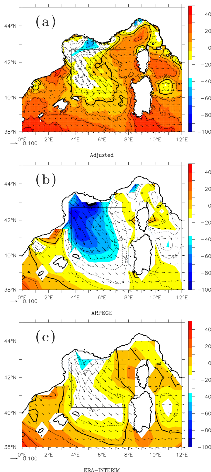
Figure 10. Maps of the annual net heat flux (shades, \text{W m}^{-2} ) and wind stress (arrows, \text{N m}^{-2} and scale in the lower left corner) for (a) the adjusted flux data set, (b) the ARPEGE model, and (c) ERA-INTERIM. Period considered: 1 August 2012 to 31 July 2013. Contour intervals are 10 \text{ W m}^{-2} . The wind stress is represented every 10 grid points.
