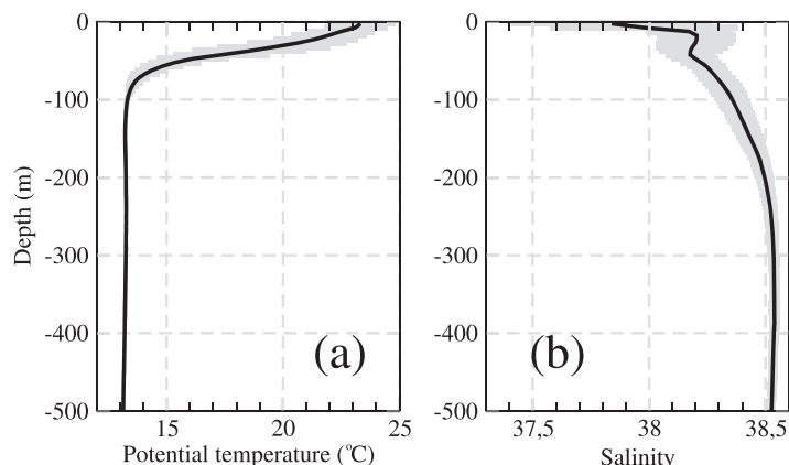
Figure 2. (a) Area mean temperature (in °C) and (b) salinity profiles from the CTDs collected within the test area (see Figure 1) during the MOOSE 2012 hydrological network with standard deviations in grey.
