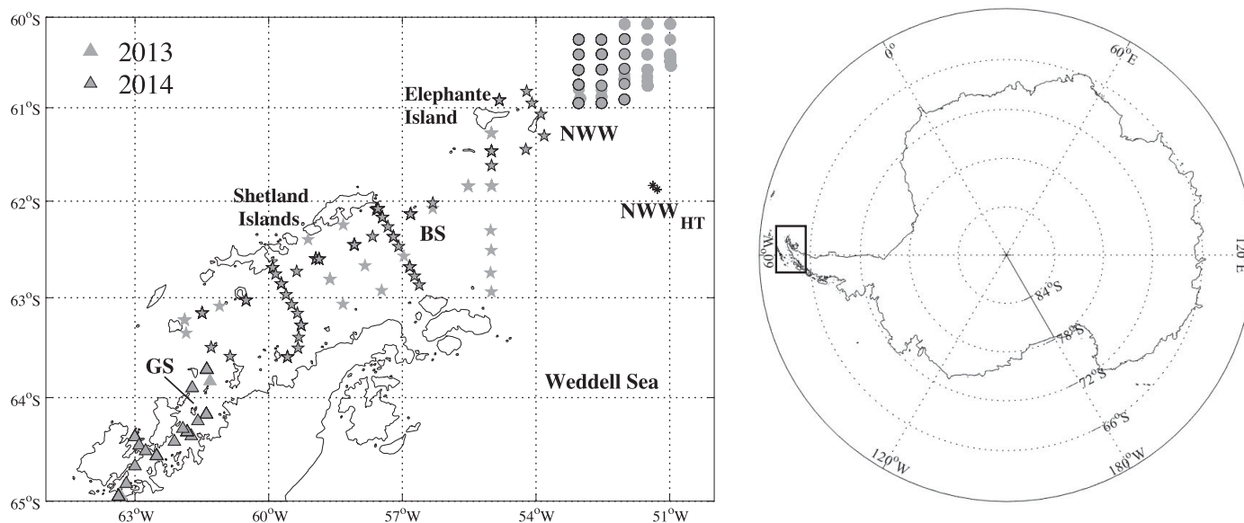
Figure 1. Geographic locations of the sampling stations in the Gerlache Strait (GS, triangles), Bransfield Strait (BS, stars), and northwestern Weddell Sea (NWW, circles). NWW HT denotes “high transparency,” with two stations sampled in 2014 (asterisks). In GS, BS, and NWW, most of the stations of 2013 were sampled in 2014 and are indicated with the edge markers in black.
