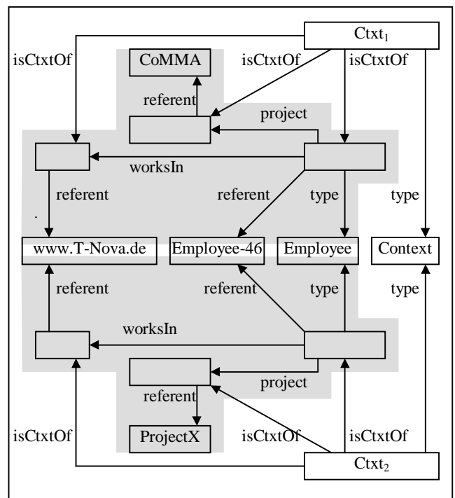
Figure 6. Two contexts about the resource Employee-46.
