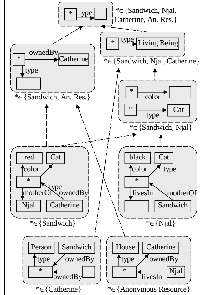
Figure 4. The concept hierarchy associated to descriptions of length 1 extracted from the RDF graph of Figure 3.
