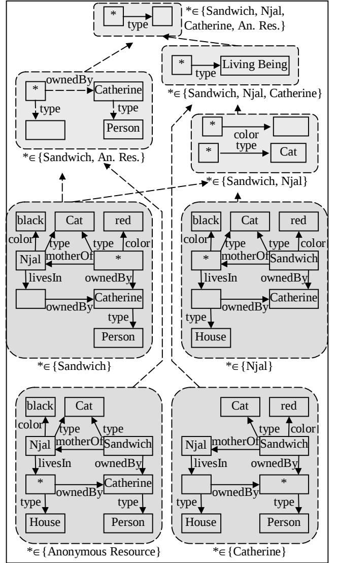
Figure 7. S_2 resulting from the index file of Figure 6.
