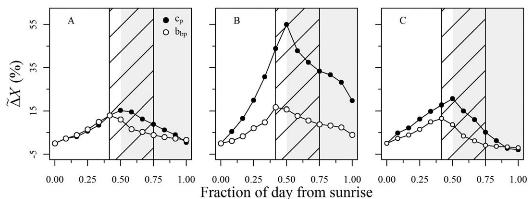
Figure 12. Average \bar{\Delta}c_p (black dots) and \bar{\Delta}b_{bp} (open circles) during situations of (a) oligotrophy, (b) bloom development, and (c) bloom decline. The hashed area is the cell division period and the shaded area is nighttime.
