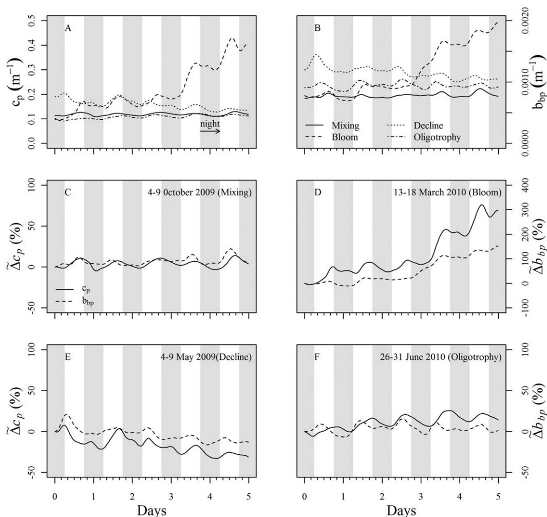
Figure 5. Examples of 5 day time series of (a) c_p and (b) b_{bp} chosen within each of the four seasons (as indicated in Figure 5b). The corresponding daily percent variation ( \Delta c_p and \Delta b_{bp} ) are displayed in Figures 5c–5f. Gray areas indicate nighttime.
