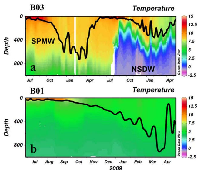
Figure 4. Time series of temperature (°C) in the upper 1000 m observed by the B03 and B01 floats, respectively. The black lines represent the density-based mixed layer depth (MLD 0.03 ). SPMW = Subpolar Mode Water; NSDW = Norwegian Sea Deep Water.
