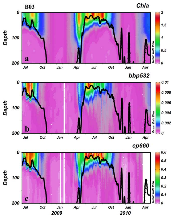
Figure 5. (a) Time series of chlorophyll-a concentration (units mg m -3 ); (b) particle backscattering coefficient at 532 nm (b bp (532)) (m -1 ); and (c) particle beam attenuation coefficient at 660 nm (c p (660)) (m -1 ) in the upper 200 m, observed by the B03 float. The black lines represent the density-based mixed layer depth (MLD 0.03 ).
