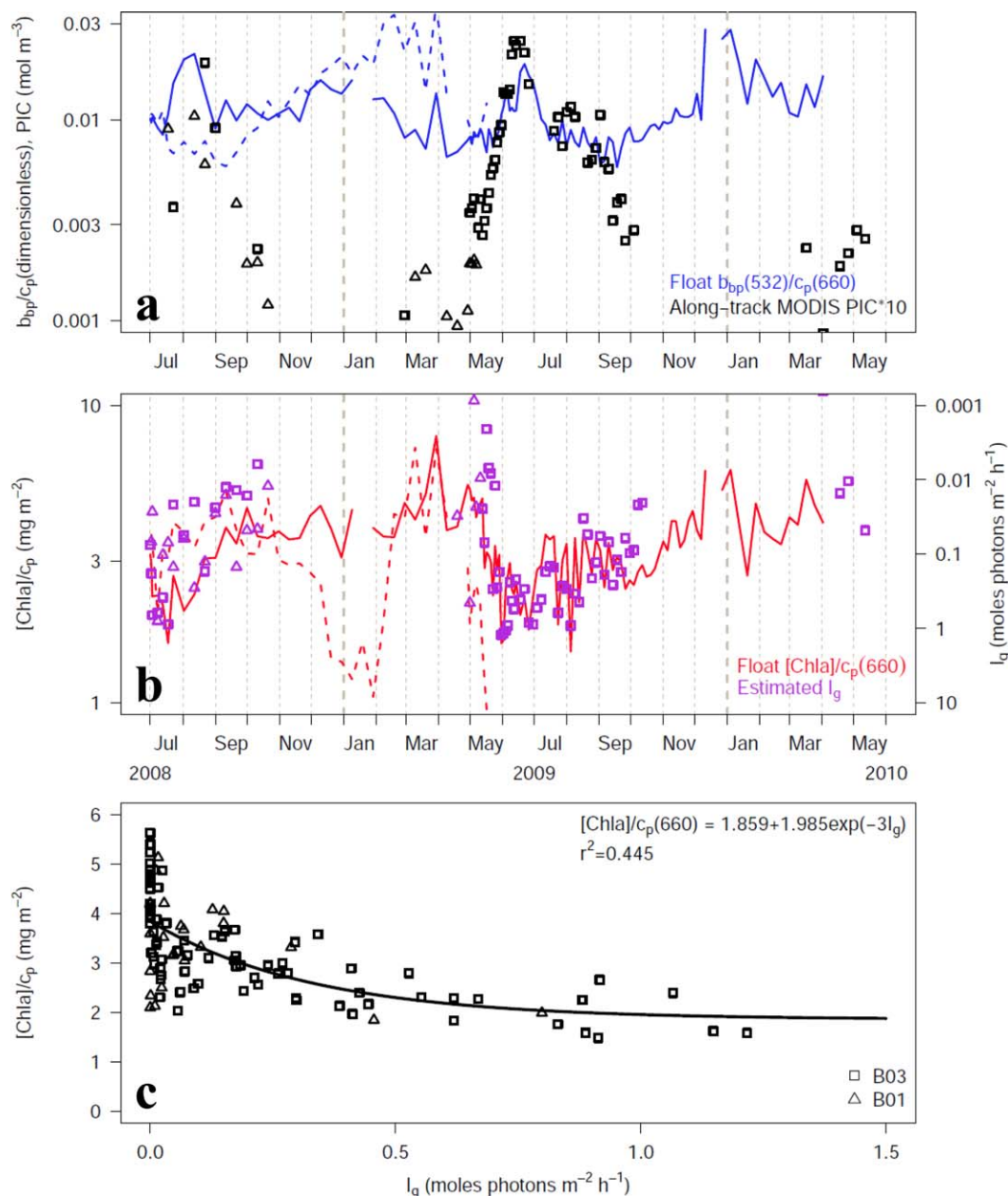
Figure 10. (a) Time series of float-measured b_{bp}(532)/c_p(660) (dimensionless) and MODIS remotely sensed particulate inorganic carbon (PIC) concentration ( \text{mol m}^{-3} ). Note that PIC has been multiplied by ten, in order to share the left axis with b_{bp}/c_p . (b) Time series of float-measured [\text{Chla}]/c_p(660) ( \text{mg m}^{-2} ) and estimated growth irradiance ( I_g ) ( \text{moles photons m}^{-2} \text{ h}^{-1} ). Note that the right axes for I_g are reversed. (c) Scatter plot between I_g and [\text{Chla}]/c_p(660) ; the black line represents the best-fit regression line.
