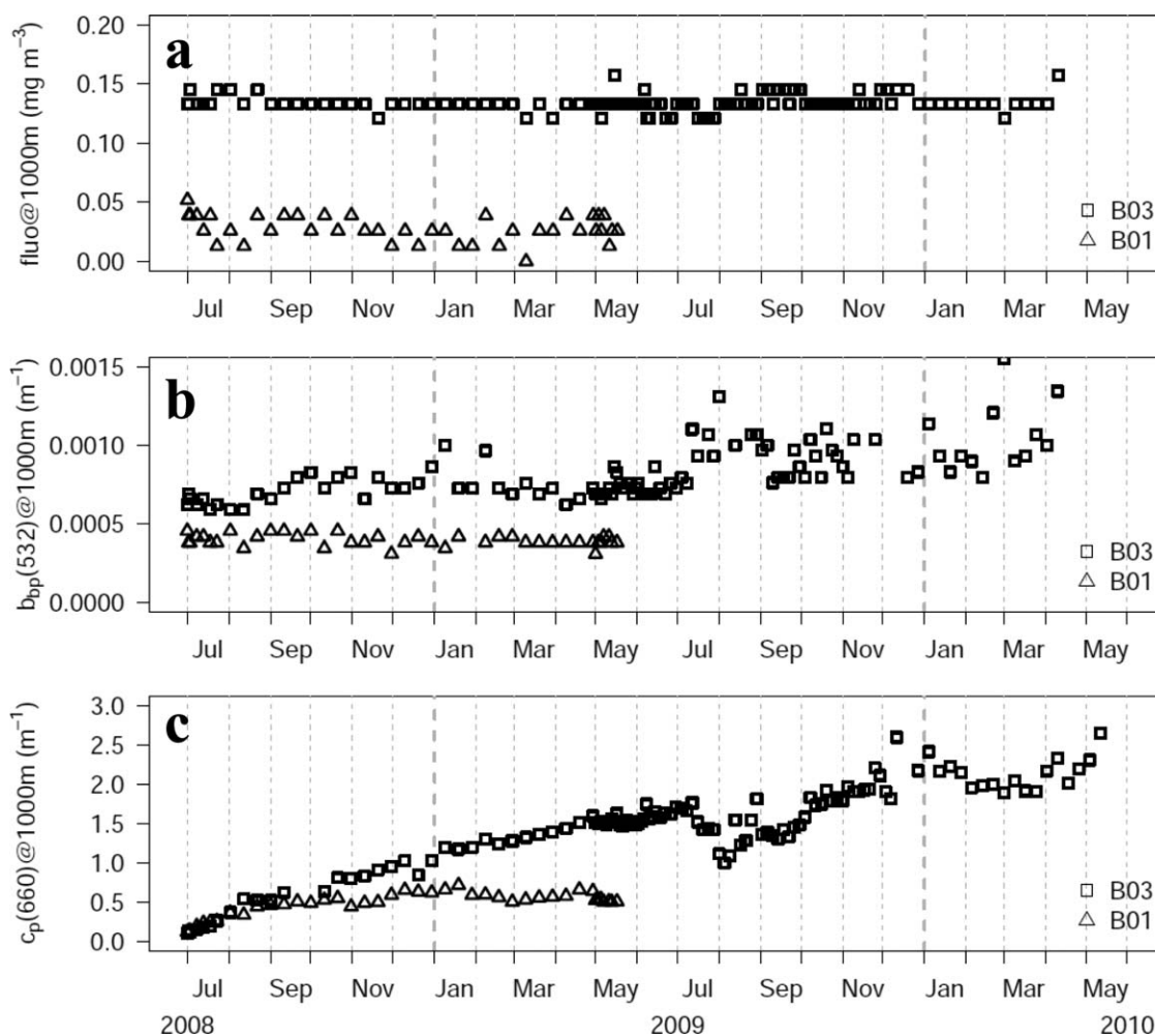
Figure 2. (a) Time series of chlorophyll-a fluorescence, (b) b_{bp}(532) , and (c) c_p(660) at the parking depth (1000 m). The squares and triangles represent the values recorded by the B03 and B01 floats, respectively.
