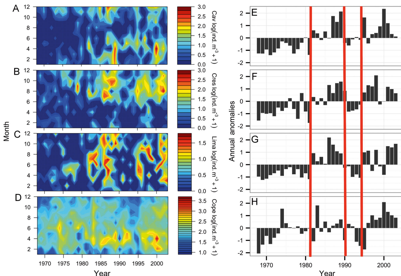
Fig. 5. Seasonal and inter-annual variability of (A) Cavoliniidae (Cav), (B) Creseidae (Cres), (C) Limacinidae (Lima) and (D) copepod (Cope) abundances ( \log \text{ind. m}^{-3} ), and standardised annual anomalies of the abundances of (E) Cavoliniidae, (F) Creseidae, (G) Limacinidae and (H) copepods at Point B. Red lines separate alternating periods of high and low abundances
