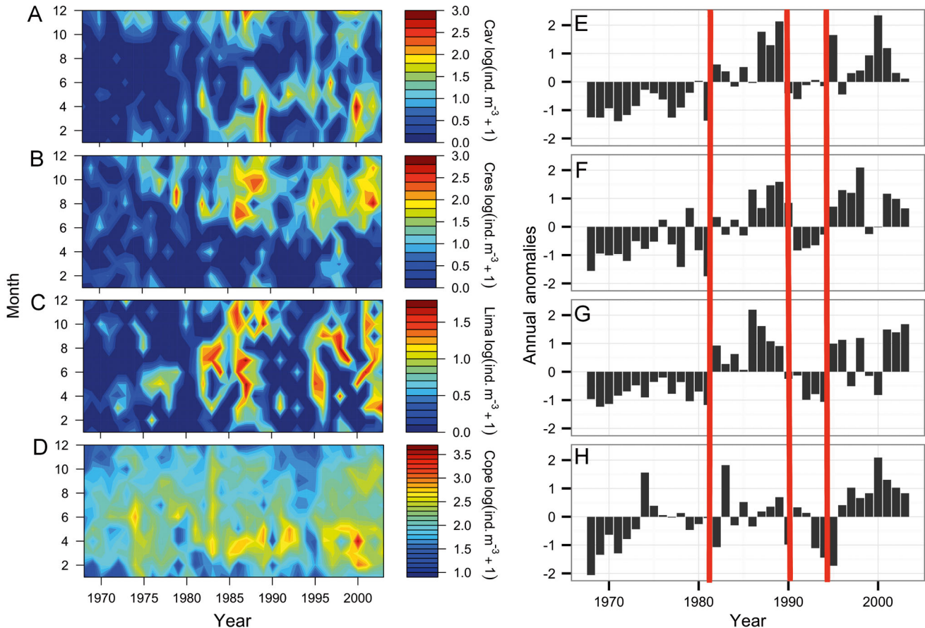
Fig. 5. Seasonal and inter-annual variability of (A) Cavoliniidae (Cav), (B) Creseidae (Cres), (C) Limacinidae (Lima) and (D) copepod (Cope) abundances ( \log \text{ind. m}^{-3} + 1 ), and standardised annual anomalies of the abundances of (E) Cavoliniidae, (F) Creseidae, (G) Limacinidae and (H) copepods at Point B. Red lines separate alternating periods of high and low abundances
