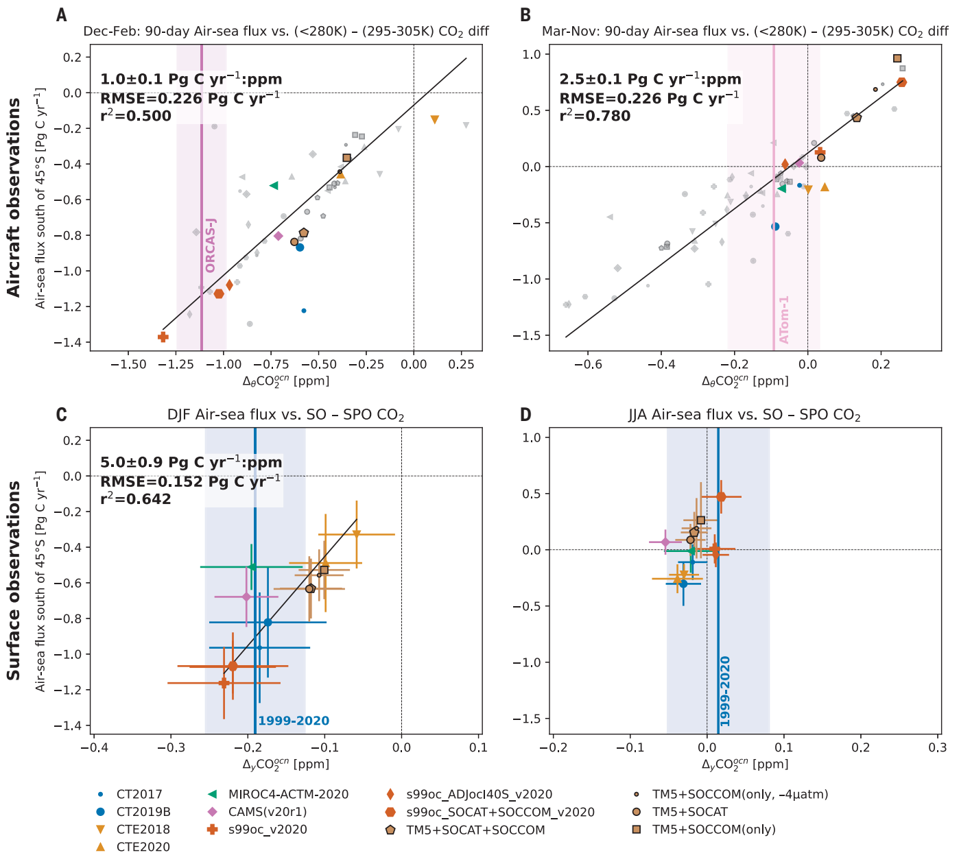
Fig. 3. Emergent constraints on air-sea fluxes south of 45°S. (A and B) 90 day–mean air-sea fluxes south of 45°S versus \Delta_{\theta}\text{CO}_2^{\text{cn}} from model simulations (see SM) replicating aircraft observations collected during (A) December to February and (B) March to November. Colored vertical lines show an observed value of \Delta_{\theta}\text{CO}_2 [ORCAS during January in (A) and ATom-1 in (B)] corrected for land and fossil fuel influence, with shading indicating both analytical uncertainty and model spread in the correction (see SM); colored points highlight the model samples from these particular campaigns, while gray points show data from other campaigns in the (A) December to February or (B) March to November timeframe. Figures S10 and S11 show similar plots for each individual aircraft campaign. (C and D) Seasonal-mean surface fluxes versus \Delta_{\gamma}\text{CO}_2^{\text{cn}} computed
