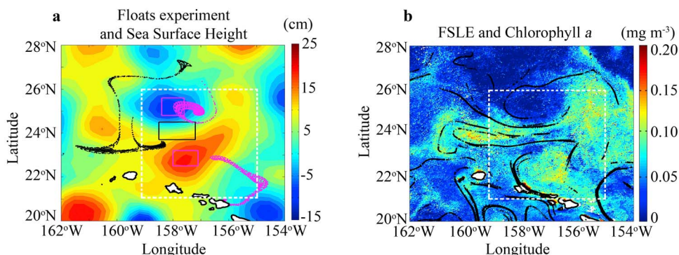
Figure 7. (a) Backward trajectory model designed to identify the source of the waters released in the cyclone and anticyclone (pink rectangles) and frontal zone (black rectangle). Floats were advected backward for 30 days using the AVISO-derived surface geostrophic velocities. (b) Finite-size Lyapunov exponents (FSLE) maxima superimposed on chlorophyll a from MODIS (8-day composite centered on 5 August 2008) representing the location of large stretching. White dashed rectangles delimit the area presented in Figure 4.
