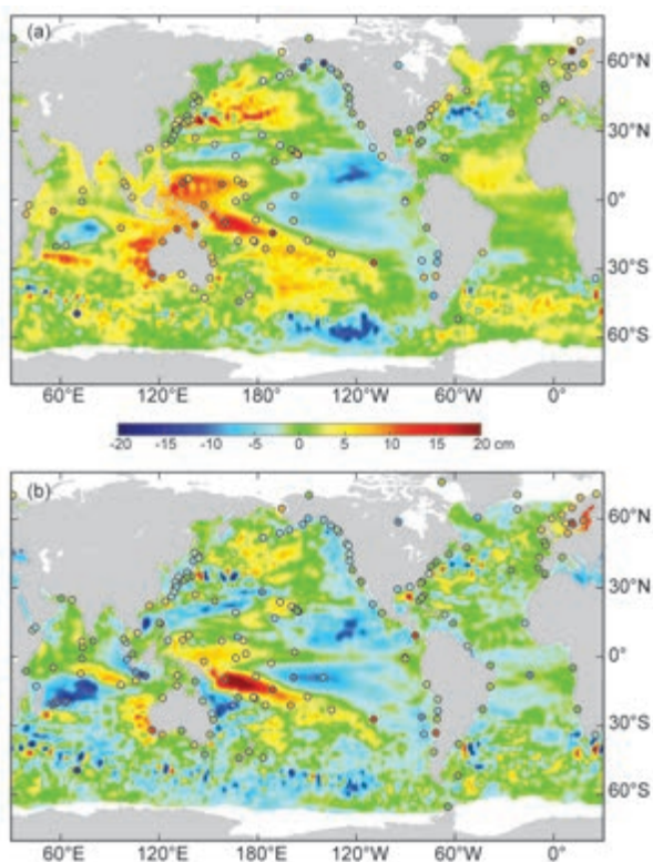
FIG. 3.26. (a) The 2011 SSH anomaly ( Ssalto/Duacs product with anomaly, cm) from the 1993–2011 base period is compared to the 2011 anomaly computed for tide gauge data (dots) obtained from the University of Hawaii Sea Level Center ( http://uhslc.soest.hawaii.edu/ ). (b) The difference between 2011 and 2010 annual means (cm).
