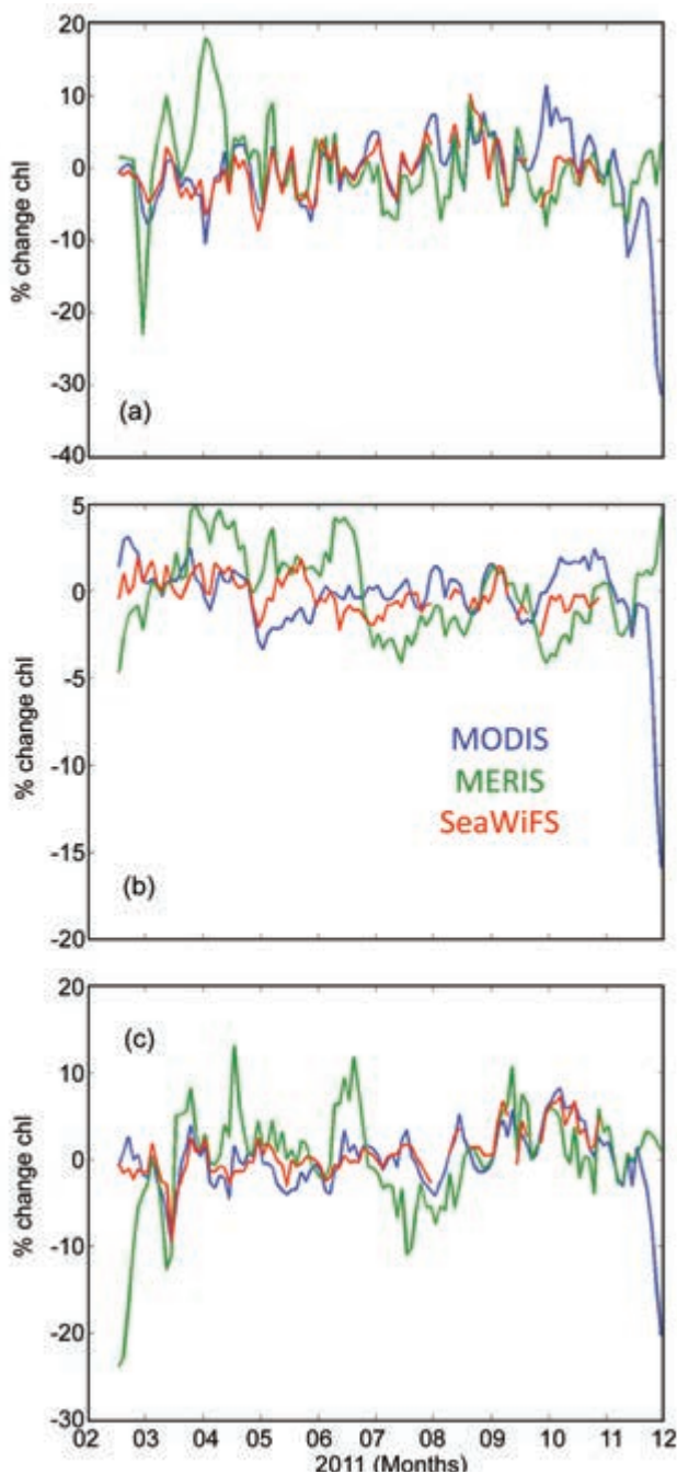
FIG. 3.38. Monthly anomalies for \log_e(\text{Chl}) averaged over (a) the cool region of the Northern Hemisphere oceans (mean SST < 15^\circ\text{C} ), (b) the warm ocean (mean SST > 15^\circ\text{C} ), and (c) the cool region of the Southern Hemisphere oceans for the SeaWiFS (red), MODIS (blue), and MERIS (green) data records. Figure 3.36 shows the location of the mean 15^\circ\text{C} isotherm. Values are calculated from 1^\circ gridded monthly log-transformed anomalies using each mission's climatology following procedures from previous State of the Climate reports and other publications (e.g., Behrenfeld et al. 2006; 2009; O'Malley et al. 2010; Siegel et al. 2011).
