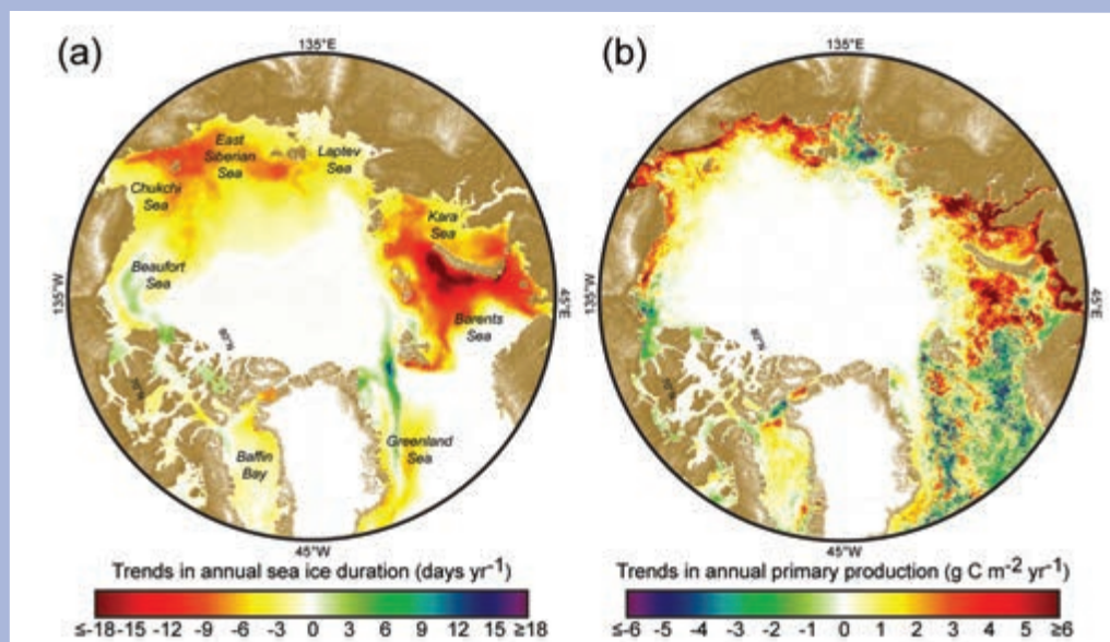
FIG. SB5.3. Trends in annual sea ice duration (days yr -1 ) and total annual net primary production (g C m -2 yr -1 ) across the Arctic Ocean and its adjacent shelf seas from 1998 to 2009 (Frey et al. 2011). Annual sea ice persistence data (based on a 15% sea ice concentration threshold) are derived from SSM/I passive microwave radiances (Cavalieri et al. 2008) and primary production data are from Arrigo and van Dijken (2011).
