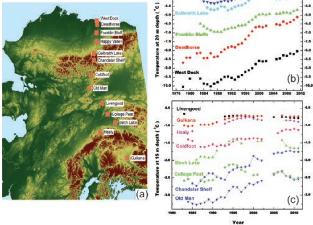
FIG. 5.14. (a) Location of sites where permafrost temperature was measured at (b) 20 m below the surface at locations from north to south across the North Slope of Alaska in the continuous permafrost zone, and (c) at 15 m below the surface in the Brooks Range and in interior Alaska. Note the higher permafrost temperatures in (c) interior Alaska than on the (b) North Slope due to the warmer climate of the interior.
