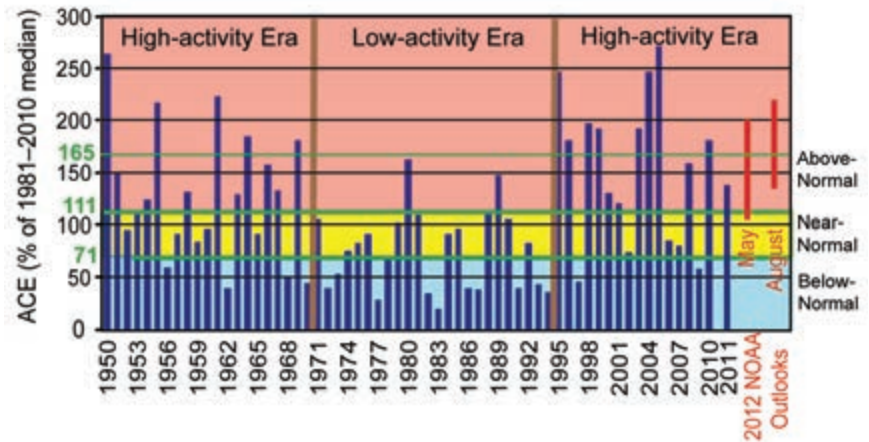
Fig. 4.8. NOAA's ACE index expressed as percent of the 1981–2010 median value. ACE is calculated by summing the squares of the six-hourly maximum sustained wind speed (knots) for all periods while the storm has at least tropical storm strength. Red bars show NOAA's predicted ACE ranges in their May and August seasonal hurricane outlooks. Pink, yellow, and blue shadings correspond to NOAA's classifications for above-, near-, and below-normal seasons, respectively. The 165% threshold for a hyperactive season is indicated. Vertical brown lines separate high- and low-activity eras.
