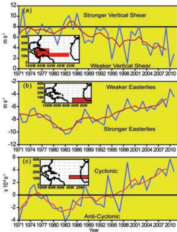
FIG. 4.16. Time series showing consecutive ASO values of area-averaged (a) 200-hPa–850-hPa vertical shear of the zonal wind ( m s^{-1} ), (b) 700-hPa zonal wind ( m s^{-1} ) and (c) 700-hPa relative vorticity ( \times 10^{-6} s^{-1} ). Blue line shows unsmoothed values and red line shows a five-point running mean of the time series. Averaging regions are shown in the insets.
