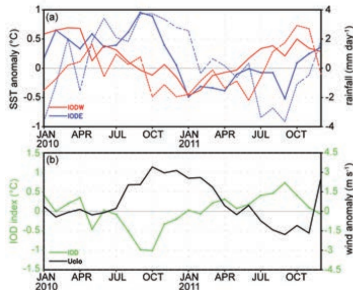
FIG. 4.38. (a) Monthly anomalies of SST ( ^\circ\text{C} , solid lines) and precipitation ( \text{mm day}^{-1} , dashed lines) in the eastern (IOD: 90^\circ\text{E} – 110^\circ\text{E} , 10^\circ\text{S} – 0^\circ ; blue lines) and western pole (IOD: 50^\circ\text{E} – 70^\circ\text{E} , 10^\circ\text{S} – 10^\circ\text{N} ; red lines) of IOD. (b) As in (a), but for the IOD index (measured by the SST difference between IODW and IODE, green line) and surface zonal wind anomaly ( \text{m s}^{-1} ) in the central equatorial IO (Ucio), from 70^\circ\text{E} – 90^\circ\text{E} , 5^\circ\text{S} – 5^\circ\text{N} , black line. The anomalies were calculated relative to the climatology over the period 1982–2010. These are based on the NCEP optimum interpolation SST (Reynolds and Chelton 2010), monthly GPCP precipitation analysis ( http://precip.gsfc.nasa.gov/ ), and JRA-25 atmospheric reanalysis (Onogi et al. 2007).
