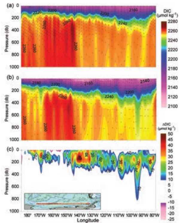
FIG. 3.32. Sections of dissolved inorganic carbon across the Pacific sector of the Southern Ocean (S4P) in (a) Feb–Apr 2011, (b) Feb–Mar 1992, and (c) the 2011 minus 1992 difference ( \mu\text{mol kg}^{-1} ). The 1992 data are from Chipman et al. (1997).
