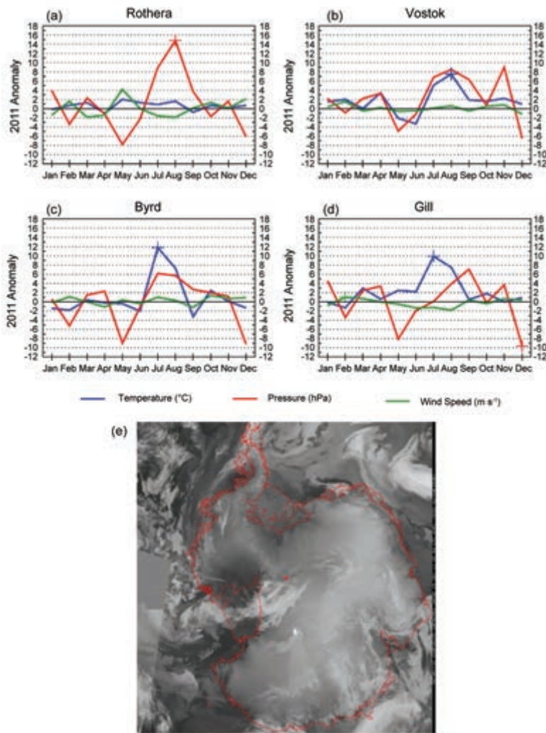
Fig. 6.5. (a)–(d) 2011 Antarctic climate anomalies at four representative stations (two staffed, two automatic). Monthly mean anomalies for temperature ( ^{\circ}\text{C} ), MSLP (hPa), and wind speed ( \text{m s}^{-1} ) are shown, with plus signs (+) denoting record anomalies for a given month at each station in 2011. Climatological data start in 1976 for Rothera, 1958 for Vostok (with some gaps), 1980 for Byrd, and 1985 for Gill. The base period for calculating anomalies was 1981–2010 for the staffed stations, and the full period of observation for the automatic stations. (e) Satellite mosaic of thermal-band emission on 25 December 2011, date of an all-time record high temperature at South Pole ( -12.3^{\circ}\text{C} ). The red dot shows the location of Amundsen-Scott South Pole station.
