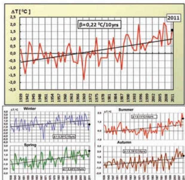
FIG. 7.32. Annual and seasonal mean temperature anomalies (°C) averaged over the Russian Federation.
