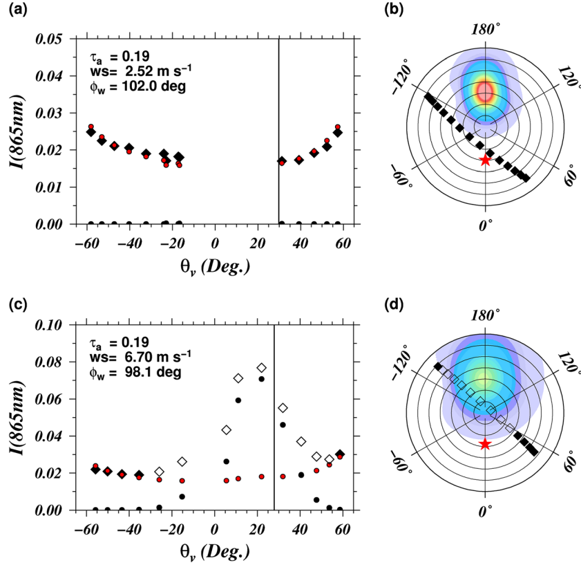
Figure 4. Examples of application of the POLAC-glint algorithm to PARASOL data acquired on 5 May 2006 over the Mediterranean sea. (a) Top of atmosphere radiance at 865 nm measured by PARASOL for a ground target that is not contaminated by sunglint (black diamonds) and radiance simulated by POLAC algorithm (red circles) and Cox and Munk model (black circle). (b) Polar diagram showing geometries of the multidirectional acquisition of PARASOL. Cox and Munk model computation of the sunglint is superimposed (colored pattern). (c) and (d) Similar to Figures 4a and 4b for a ground target that is contaminated by sunglint (white diamonds). The viewing angle is negative when the relative azimuth angle is between 90^\circ and 270^\circ . The Sun position is illustrated by a vertical line in Figures 4a and 4c and by a red star in Figures 4b and 4d. The color scale used is the same as the one used in Figure 1.
