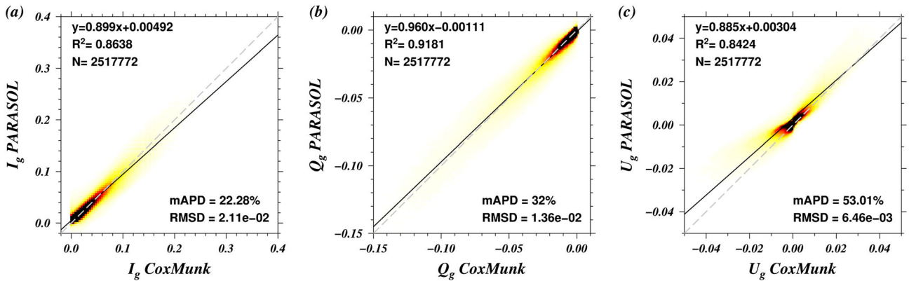
Figure 8. Comparison between the sunglint component of the Stokes parameters (a) I_g , (b) Q_g , and (c) U_g (dimensionless) simulated using Cox and Munk model at the top of the atmosphere at 670 nm ( x -axis) and the sunglint Stokes parameters retrieved using POLAC-glint algorithm applied to the PARASOL data acquired over the world on 5 May 2006. N is the number of data considered, mAPD is the median of the absolute percentage difference (in %) and RMSD is the root-mean-square difference.
