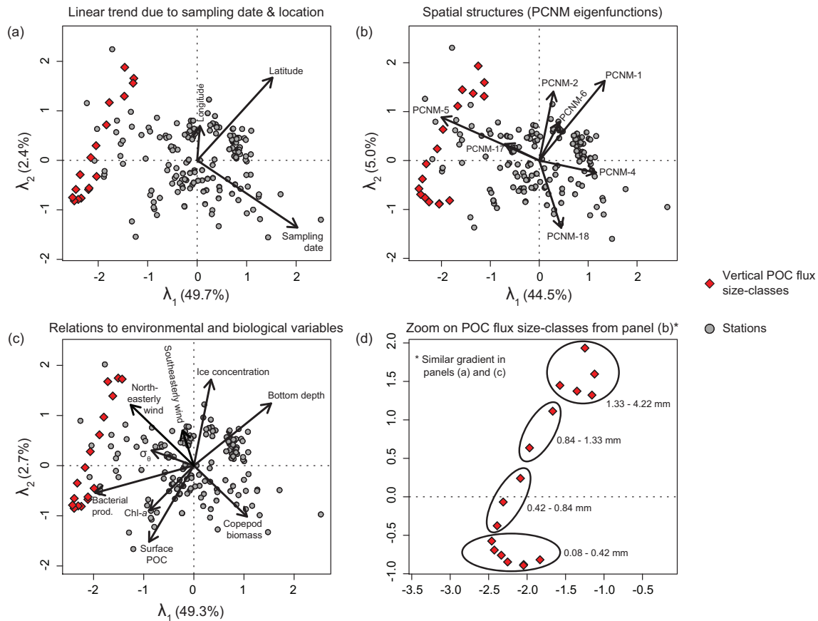
Fig. 14. Ordination plots of axes I and II from redundancy analyses (RDAs) conducted between the 17 vertical POC flux size classes (i.e., used as “species”), the 154 station locations, and the three reduced models obtained from the forward selection procedures: (a) linear trend due to sampling date and location, (b) variance from the PCNM sinusoidal-like waveform functions, and (c) trend induced by the set of significant environmental and biological variables. The list of all biophysical variables available for the present study is presented in Table 4. Panel (d) is a zoom on the ordination gradient of POC flux size classes (expressed in equivalent spherical diameter) as obtained from the PCNM RDA, but the gradient is similar in panels (a) and (c). Details from the forward selection procedures are presented in Table 3. Spatial patterns corresponding to the PCNM functions and associated canonical axes are presented in Fig. 15. PCNM: principal coordinates of neighbor matrices (Borcard et al., 2011).
