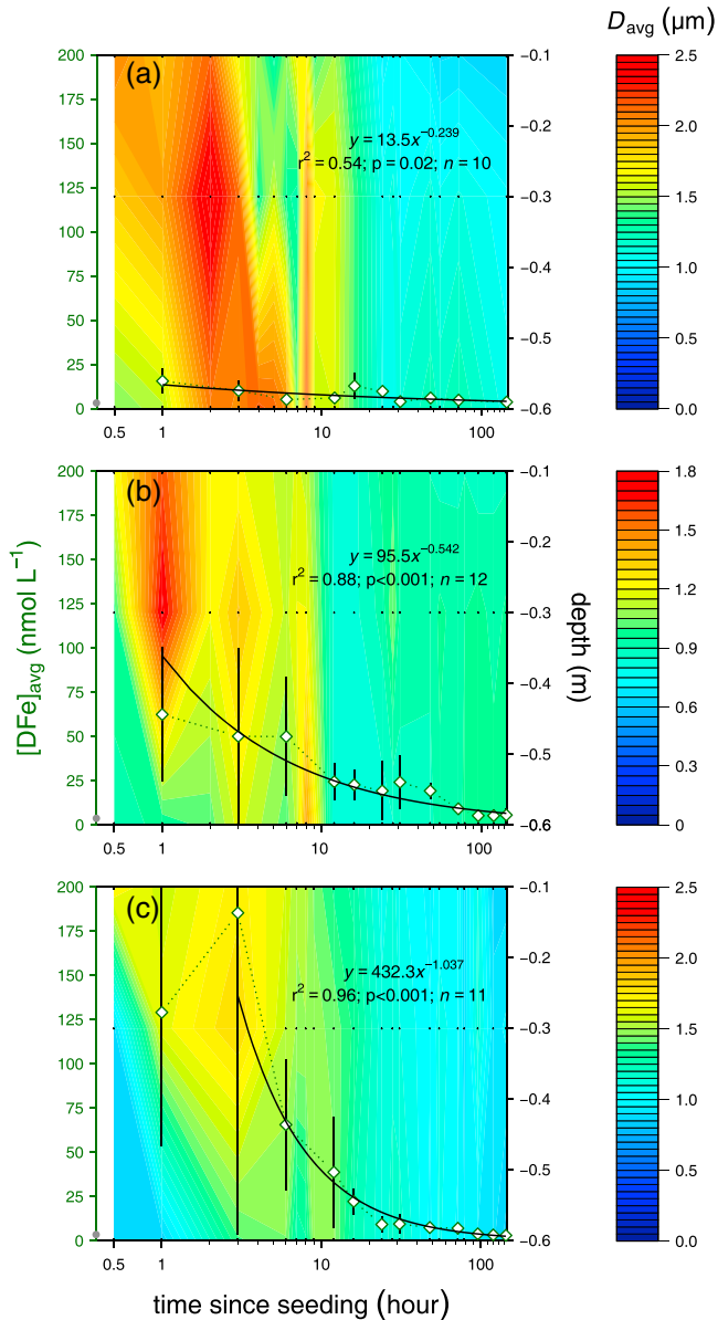
Figure 1. The temporal evolution of the mean number diameter ( D_{\text{avg}} ) profile from 0.1 to 0.6 m depths measured in (a) May, (b) October, and (c) February. The superimposed dotted curves and the white diamonds correspond to the temporal evolution of the [\text{DFe}]_{\text{avg}} ( [\text{DFe}] averaged over the three sampling depths). Gray circles on the y axis represent the initial values of [\text{DFe}]_{\text{avg}} . Black curves correspond to the power law model used to calculate DFe loss rates. The error bars represent the standard deviation for the values measured at the three sampling depths. The D_{\text{avg}} scale in Figure 1b has been changed for clarity. Note the logarithmic x-scale.
