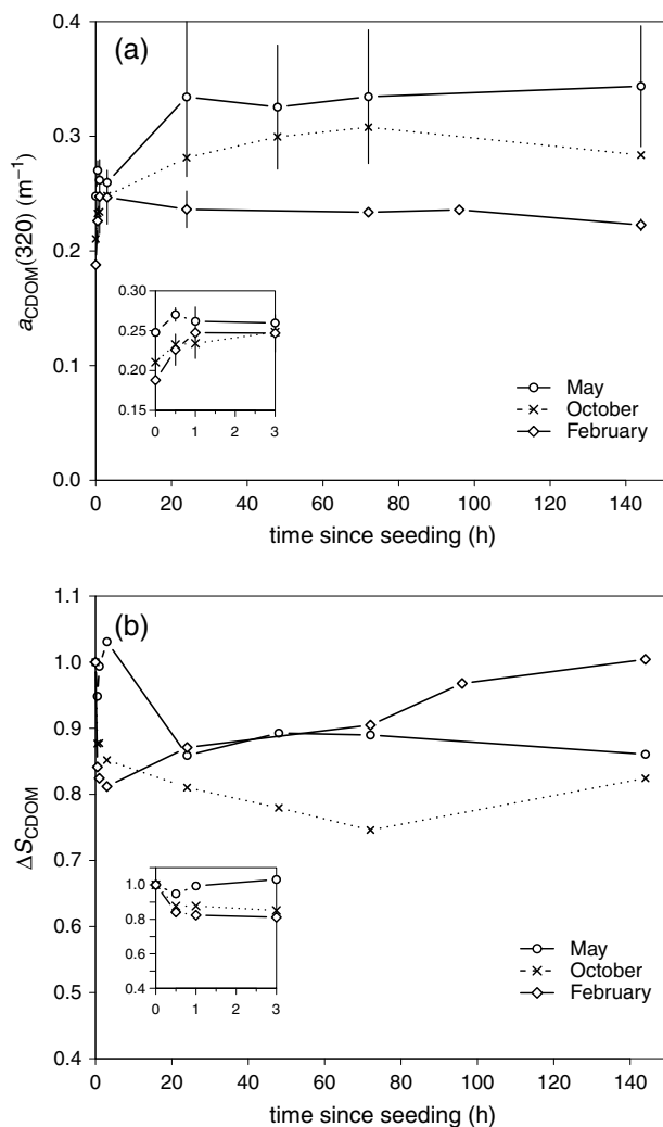
Figure 2. The temporal evolution of (a) CDOM absorption at 320 nm ( a_{\text{CDOM}(320)} ; \text{m}^{-1} ) and (b) the spectral slope of CDOM ( S_{\text{CDOM}} ) in relation to the initial value ( \Delta S_{\text{CDOM}} = S_{\text{CDOM}(T_x)} / S_{\text{CDOM}(\text{initial})} ), both averaged over the three sampling depths. Insets provide the zoom for the 0–3 h period. For clarity, the error bars in October have not been added in Figure 2a. Numbers were compared between the three seasons using a one-way analysis of variance and a Student's t test ( \alpha=0.05 ). Results indicated that means are significantly different from each other.
