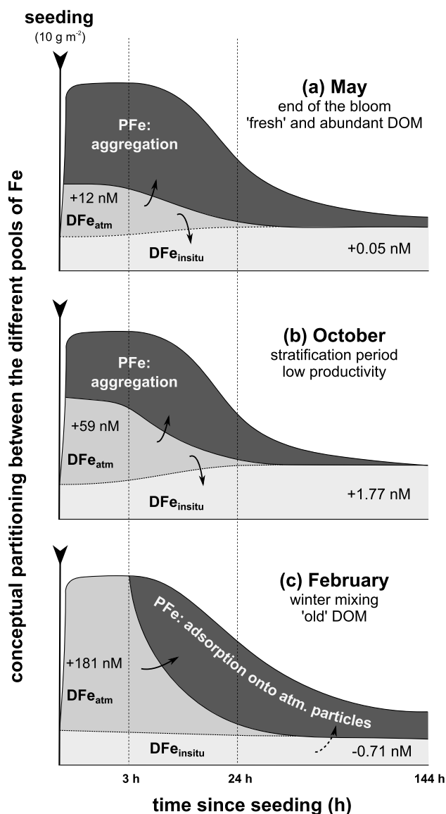
Figure 4. Conceptual schema of the dynamic exchanges between the iron phases following the seeding during (a) May, (b) October, and (c) February. DFe_{atm} : dark gray; DFe_{insitu} : light gray; the Fe adsorbed on or included by the particle population (atmospheric particles and organic-mineral aggregates): black. The definition of DFe_{atm} and DFe_{insitu} can be found in the text (section 4.2.).
