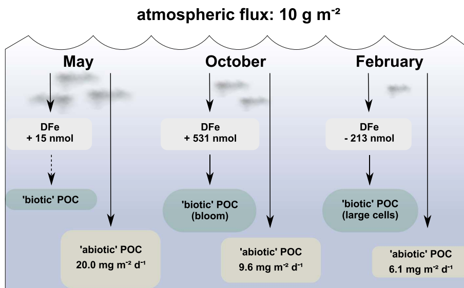
Figure 6. “Abiotic POC” export, the change in DFe stock six days after each atmospheric deposition event, and the resulting “biotic POC” export. “Abiotic” and “biotic” POC exports are discussed and defined in section 4.4.
