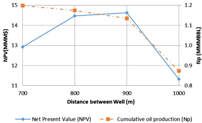
Fig. 3. Determining pilot size by sensitivity analysis.
