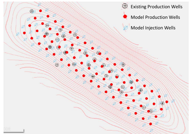
Fig. 4. Five-spot patterns in the case study reservoir.
