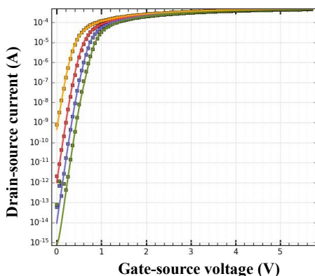
Fig. 6. Model-measurement comparison, I_{DS}(V_{GS};V_{BS}) transconductance characteristic, for 4 different bulk-source bias, for the new MV NMOS transistor. Squares are the measurement points, lines are model data.
