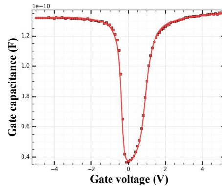
Fig. 7. Model-measurement comparison, capacitance-voltage C(V) curve, for the new MV NMOS transistor. Squares are the measurement points, lines are model data.
