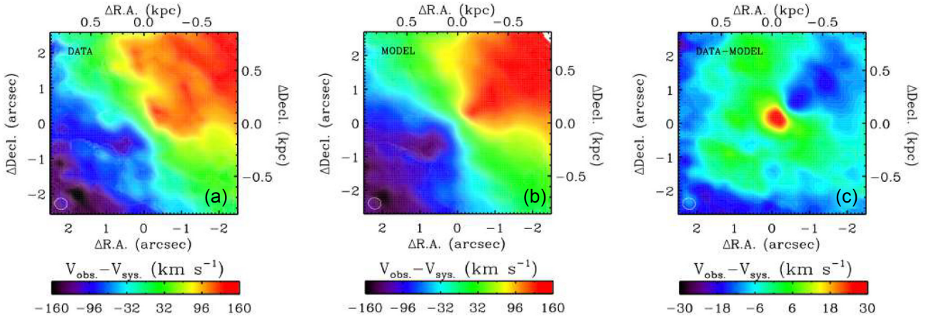
Figure 11. Same as Fig. 6 but for ^{12}\text{CO}(1-0) . The best-fitting KinMS model is the one shown in panel (c) of Fig. 10.
