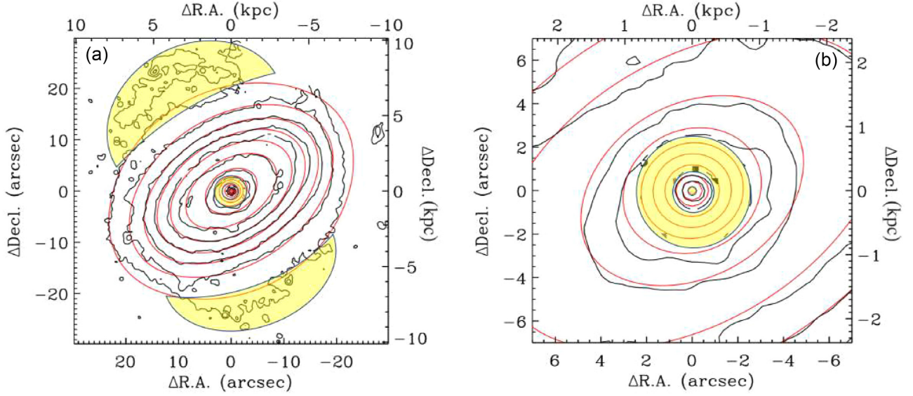
Figure 8. The comparison between the HST/F547M photometry of NGC 7469 (black) and its corresponding best-fitting MGE model (red) at the same radii, which illustrate the whole galactic scale 60 \text{ arcsec} \times 60 \text{ arcsec} ( \approx 20 \times 20 \text{ kpc}^2 , panel a) and the zoom-in of 14 \text{ arcsec} \times 14 \text{ arcsec} ( \approx 4.6 \times 4.6 \text{ kpc}^2 , panel b) FOV. Yellow regions are the pixel excluded during the MGE fit.
