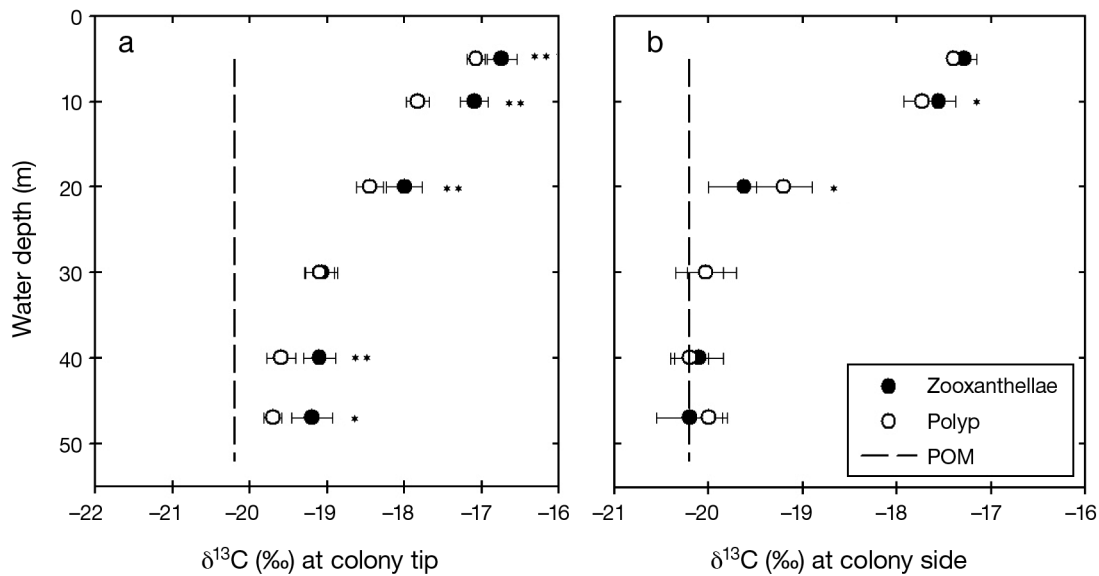
Fig. 2. Madracis spp. \delta^{13}\text{C} of zooxanthellae and host polyp for (a) tip and (b) side of colony positions versus water depth. Error bars are SE of mean values. Vertical dashed line gives estimate for \delta^{13}\text{C} of POM. * p < 0.05 and ** p < 0.005 (paired t -test for tips and side of colony positions)
