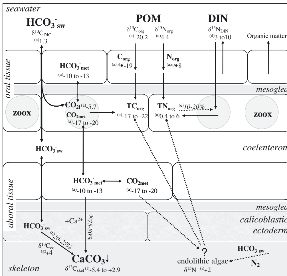
Fig. 4. Madracis spp. Model of pathways and fluxes of carbon and nitrogen contributing to stable isotope fractionation and composition of total organic carbon and nitrogen ( \text{TC}_{\text{org}} and \text{TN}_{\text{org}} ) as measured in the tissues of branching Madracis spp. The model was combined and modified from models for carbon acquisition (Furla et al. 2000a), carbon isotope fractionation (Muscatine et al. 1989) and nitrogen flux and isotope fractionation (Heikoop et al. 1998). Numbers with letters in superscript are estimates for \delta^{15}\text{N} or \delta^{13}\text{C} (‰). The values were approximated from various sources as follows: (a) this study with average \delta^{13}\text{C} seawater DIC ( \delta^{13}\text{C}_{\text{DIC}} ), seawater bicarbonate ( \text{HCO}_3^-_{\text{sw}} ), metabolic \text{CO}_2 ( \text{CO}_{2\text{met}} ), which is similar to \delta^{13}\text{C} of animal tissue (Muscatine et al. 1989), while metabolic bicarbonate ( \text{HCO}_3^-_{\text{met}} ) is enriched by \sim 7\% relative to \text{CO}_{2\text{met}} and vice versa. The same fractionation factor of 7‰ was applied between \delta^{13}\text{C}_{\text{DIC}} and inorganic \text{CO}_2 ( \text{CO}_{2\text{i}} ), which is taken up by zooxanthellae (zoox). (b) \delta^{13}\text{C} of organic carbon ( \text{C}_{\text{org}} ) is about 1‰ enriched to prey (DeNiro & Epstein 1978). In our study, we assume that POM is the major allochthonous food source. (c) Enrichment of organic \delta^{15}\text{N} ( \delta^{15}\text{N}_{\text{org}} ) by heterotrophic feeding ( \text{N}_{\text{org}} ) by an average 3.4‰ (Minagawa & Wada 1984). (d) Likely range of \delta^{15}\text{N} of seawater DIN ( \delta^{15}\text{N}_{\text{DIN}} ) (Heikoop et al. 1998). (e) Maximum of 20% of assimilated prey nitrogen has been shown to appear in endosymbiotic zooxanthellae (Piniak et al. 2003). (f) Range in skeletal \delta^{13}\text{C} ( \delta^{13}\text{C}_{\text{skel}} ) for branching Madracis spp. with a depth range similar to colonies of this study (Maier et al. 2003). (g) Equilibrium ^{13}\text{C} fractionation ( \delta^{13}\text{C} ) between aragonite and bicarbonate (Romanek et al. 1992). (h) Suggested contribution to skeletal carbon of 75 to 80% of metabolic carbon and 20 to 25% of seawater bicarbonate (Erez 1978, Furla et al. 2000a). (i) Nitrogen fixers, such as endolithic algae, have a \delta^{15}\text{N} value of \sim 2\% (France et al. 1998). A transfer of photoassimilates from endolithic algae to coral tissue (dashed arrows) may be of significance for coral metabolism in extreme situations such as in very low light environments or in bleached corals (Schlichter et al. 1995, Fine & Loya 2002). The '?' indicates that it is uncertain if endolithic algae utilize \text{CO}_2 respired by corals. Dotted line indicates optional contributions/pathways
