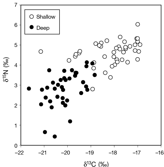
Fig. 1. Madracis spp. Correlation between \delta^{15}\text{N} and \delta^{13}\text{C} in holobiont tissue with \delta^{15}\text{N} = 16.7 + 0.69 \times \delta^{13}\text{C} ( r = 0.769 , p < 0.0001 , N = 84 ). (O) shallow (5 to 20 m), (●) deeper (30 to 47 m) water corals
