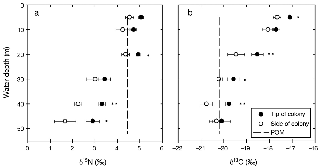
Fig. 3. Madracis spp. (a) Mean \delta^{15}\text{N} and (b) \delta^{13}\text{C} of holobiont tissue at the side and tip of branches versus water depth. Error bars are SE of mean values. Vertical dashed line gives estimate for \delta^{15}\text{N} and \delta^{13}\text{C} of POM. * p < 0.05 and ** p < 0.005 (paired t -test for tips and side of colony positions)
