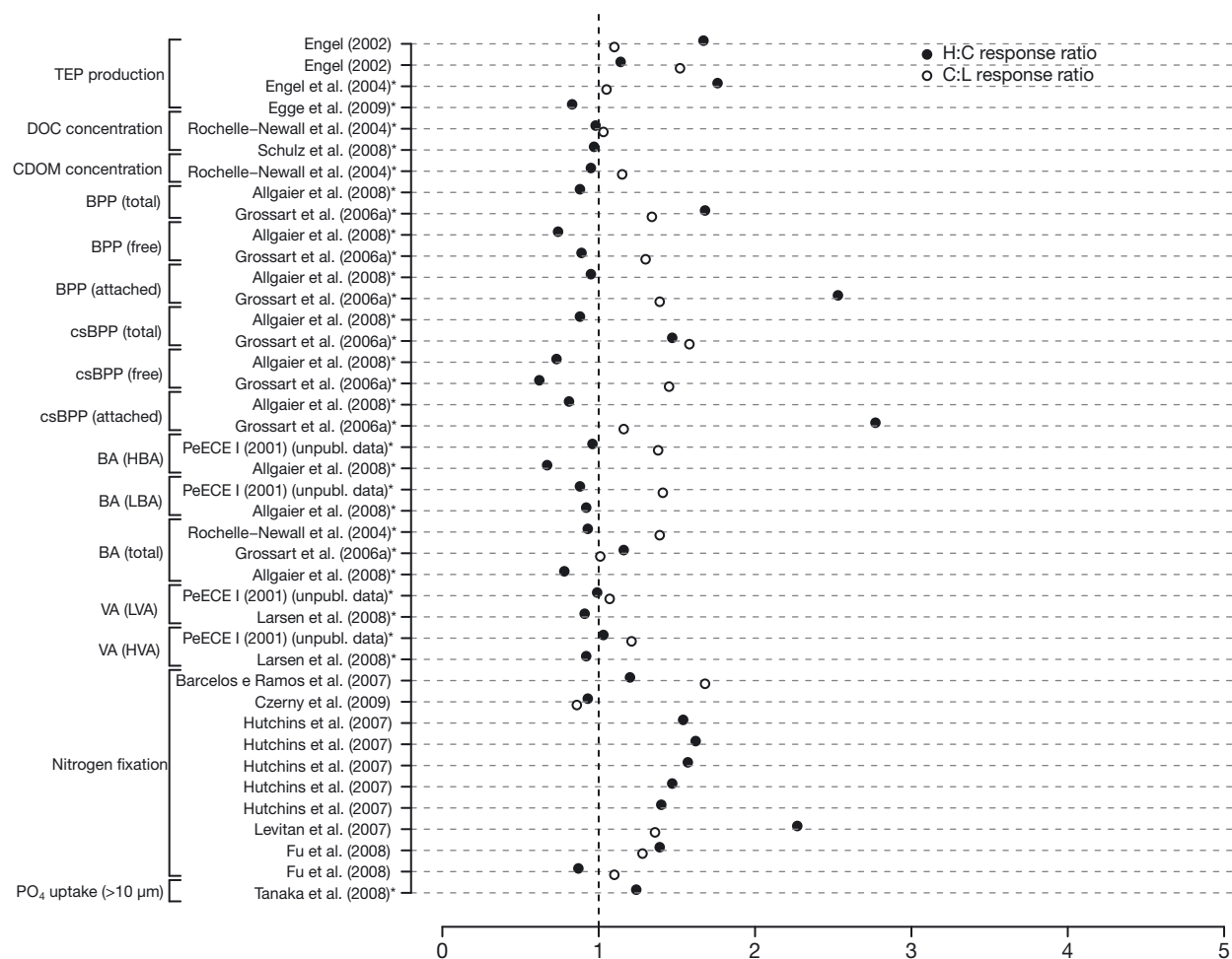
Fig. 1. Impact of ocean acidification on microbial processes and on the parameters involved. The H:C ratios, i.e. the values at high partial pressure of \text{CO}_2 ( \text{pCO}_2 ) versus the values at control \text{pCO}_2 , are shown as filled circles, whereas the C:L ratios, i.e. the values at control \text{pCO}_2 versus the values at low \text{pCO}_2 , are shown as open circles. The nitrogen fixation rate reported by Hutchins et al. (2007) at low \text{pCO}_2 was 0; hence the C:L ratios could not be calculated. Asterisks (*) indicate data collected in a mesocosm experiment during which \text{pCO}_2 was drifting (see 'Methods'). TEP: transparent exopolymer particles; DOC: dissolved organic carbon; CDOM: chromophoric or coloured dissolved organic matter; BPP: bacterial protein production; attached and free: Bacteria attached on particles or free; csBPP: cell-specific bacterial protein production; BA: bacterial abundance; HBA and LBA: abundances of high- and low-fluorescence Bacteria ; VA: viral abundance; HVA and LVA: abundances of high- and low-fluorescence viruses; APA: alkaline phosphatase activity
