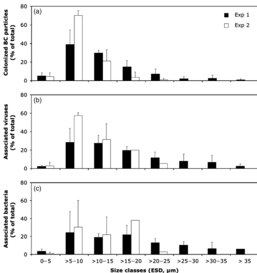
Fig. 6. Size class distribution of the percentage of BC particles with both associated viruses and bacteria (a) and contribution of BC-associated viruses (b) and bacteria (c) to the total abundance in the different BC particle size classes. Exp1, experiment 1; Exp2, experiment 2; ESD, equivalent spherical diameter. Values are given as averages \pm SD of the means of triplicate incubations.
