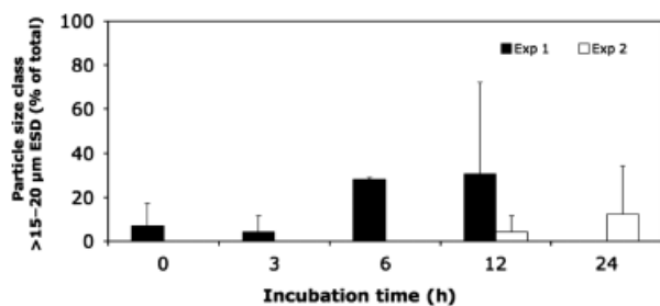
Fig. 7. Temporal changes of the percentage of BC particles with associated viruses and bacteria in the size class > 15-20 \mu\text{m} . Exp1, experiment 1; Exp2, experiment 2; ESD, equivalent spherical diameter. Values are given as averages \pm SD of the means of triplicate incubations.
