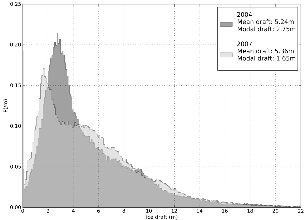
Figure 4. Overall probability density functions for the track sectors between 20°W and 70°W at about 85°N, north of Greenland, for 2004 and 2007 data. Note lower mode in 2007 and greater ridging.
