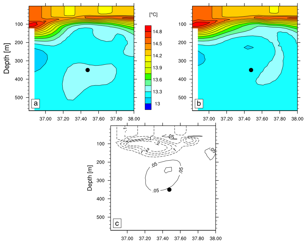
Fig. 9 Meridional transect of the Algerian Current ( 3^{\circ}23' E ) showing the vertical propagation of corrections due to trajectory assimilation on 25 January 2005: a the CTRL temperature fields ( ^{\circ}C ), b the TRAJ temperature fields ( ^{\circ}C ), and c the differences between the CTRL and TRAJ temperature fields. The black dots indicate the position of the “50769 float” before surfacing on 25 January
