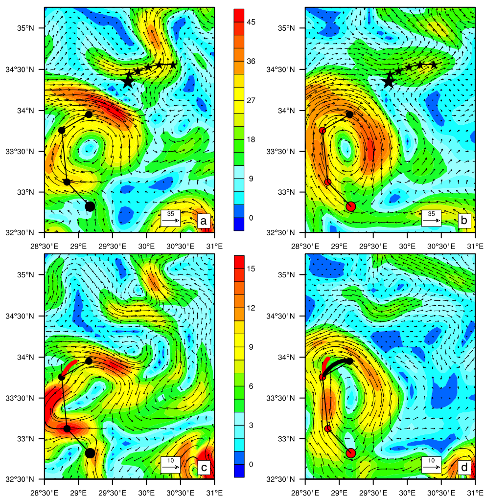
Fig. 12 Validation of TRAJ velocity fields using independent surface drifter data in the Levantine on 16 December 2006. Top panels show velocity fields (in \text{cm}^{-1} ) at 15 m depth deduced from the a CTRL and b TRAJ experiments. The lower panels present the velocity fields at 365 m depth: c CTRL with forecasted “50761 float” trajectory marked in red and d TRAJ with the corresponding predicted (red) and analyzed (black) “50761 float” trajectories. The observed “50761 float” positions (1–16 December) are marked with black (not assimilated) and red (assimilated) dots. The surface drifter (59770) positions on 16–21 December are marked with black stars. The first float and drifter positions are indicated with larger markers
