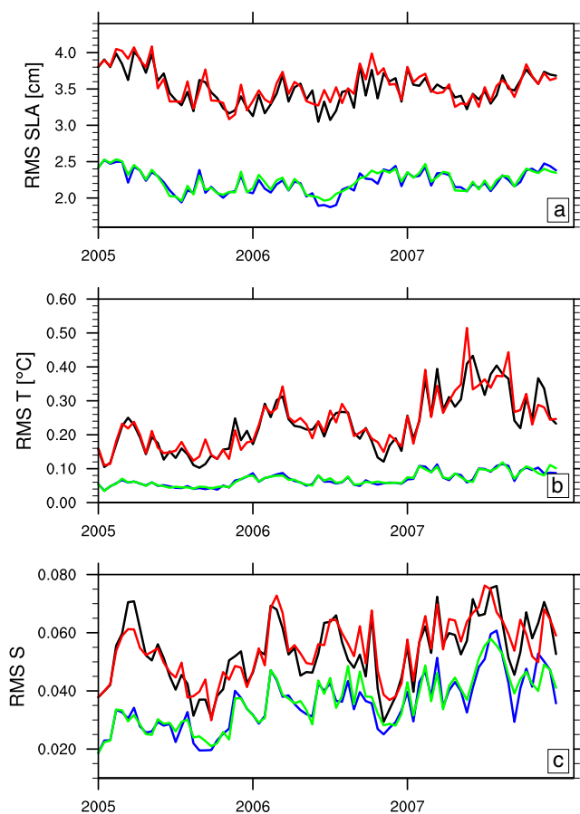
Fig. 5 Two-week Mediterranean mean RMS misfits for the CTRL ( black ) and TRAJ ( red ) experiments, as well as the RMS differences between the CTRL ( blue ) and the TRAJ ( green ) analyses and observations during 2005–2007. Top panel , sea-level anomaly RMS differences (in cm); middle panel , temperature RMS differences ( ^{\circ}\text{C} ) at 350 m depth; lower panel , salinity RMS differences at 350 m depth
