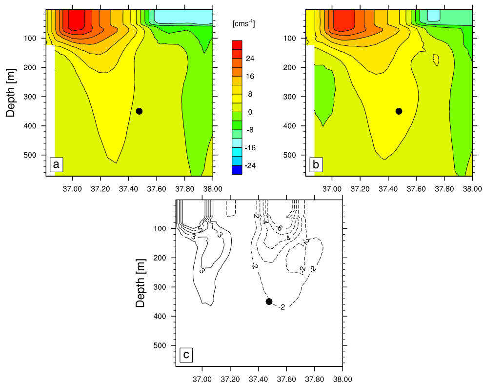
Fig. 8 Meridional transect of the Algerian Current ( 3^{\circ}23' E ) showing the vertical propagation of corrections due to trajectory assimilation on 25 January 2005: a the CTRL zonal velocity fields (in cm^{-1} ), b the TRAJ zonal velocity fields (in cm^{-1} ), and c the differences between the CTRL and TRAJ zonal velocity fields. The black dots indicate the position of the “50769 float” before surfacing on 25 January
