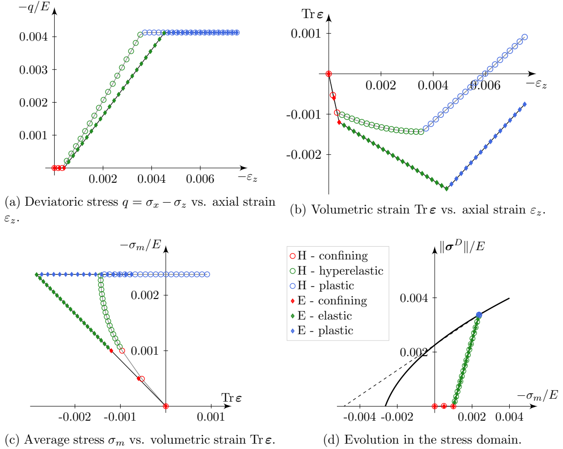
Figure 5: Comparison of the response for a triaxial compression test with a confining pressure. The different stages of the evolution are shown with different colors: hydrostatic confining ( red ), hyperelastic ( green ), and plastic ( blue ) stage. The hyperelastic response is represented with empty circles, while the elastic one with diamonds.
