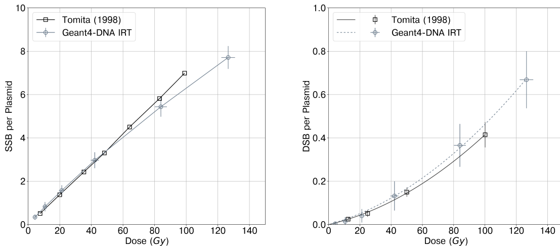
Figure 6: Dose response of SSB (left), and DSB (right). Error bars represent one standard deviation. Simulation results for SSB and DSB ( \circ ) are shown alongside Tomita's (1998) reference data ( \square ). Simulation data 2 nd order polynomial fit is shown with the dotted line.
