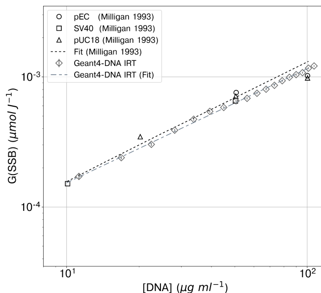
Figure 4: [DNA] ( \mu\text{g}/\text{mL} ) response of G(\text{SSB}) ( \mu\text{mol J}^{-1} ). Error bars represent statistical errors, one standard deviation. Geant4-DNA IRT results are shown ( \diamond ), experimental data are from Milligan, 1993 ( \circ , \square , \triangle ).
