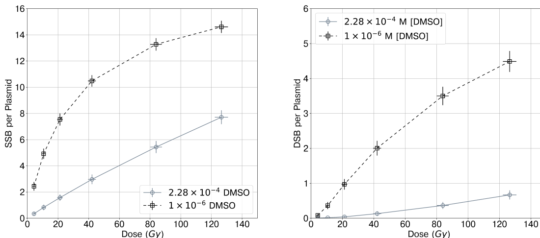
Figure 8: DMSO effect on SSB and DSB as dose increases. Error bars represent one standard deviation. 1 \times 10^{-6} M [DMSO] is shown ( \square ) against 2.28 \times 10^{-4} M [DMSO] ( \circ ), from MCTS simulations with pUC19 plasmids.
