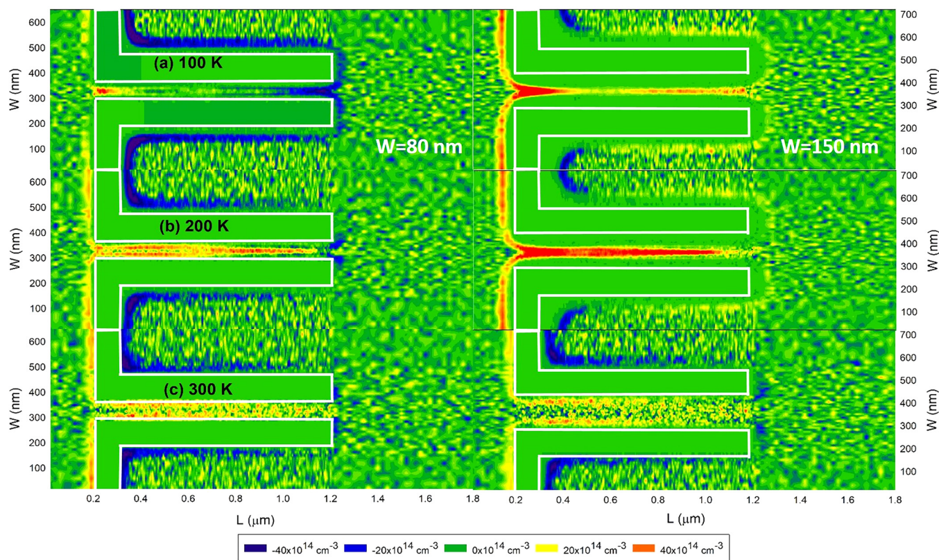
FIG. 5. Color maps of carrier concentration difference ( \Delta n ) between \pm 0.1 \text{ V} bias voltages for each SSD at three different temperatures: (a) 100, (b) 200, and (c) 300 K.
