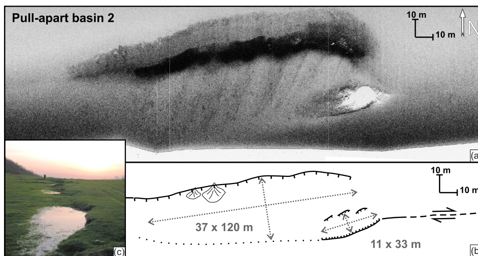
Figure 12. The side-scan sonar image exposes a basin-in-basin morphology in the shelf section (see Fig. 3 for location; profile SAR_SS03.014H). The scarp height near the fans is approximately 18 \pm 1 m. The lower-right depression is significantly smaller and may be produced during a single surface faulting event. Such depressions (sagponds) have occurred during both the 17 August and 12 November 1999 Düzce earthquake (photo by S. Pucci, sagpond on the 12 November rupture)
