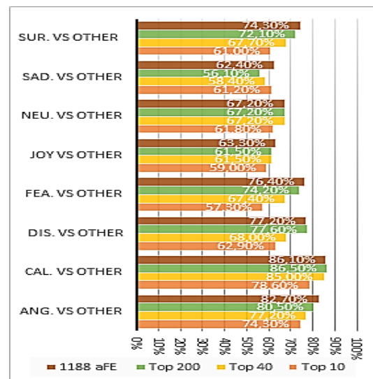
Figure 2. Accuracies obtained with various features sets
