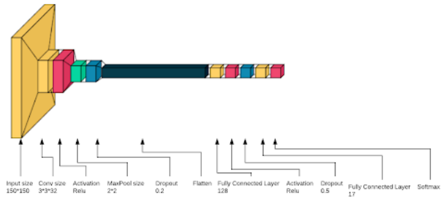
Fig. 4. Visualization of CNN architecture
