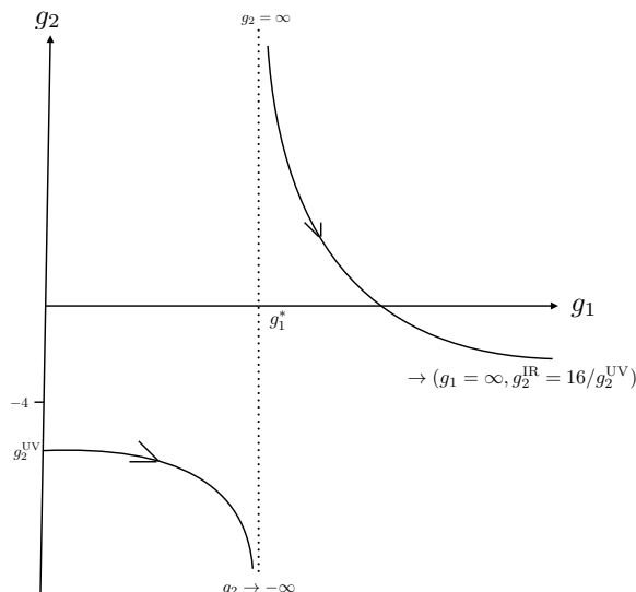
Figure 3. Sketch of the massless flow in the imaginary sinh-Gordon model from g_2^{UV} < -4 to g_2^{IR} = 16/g_2^{UV} . The value g_1^* is given in the text: g_1^* = 8\sqrt{4 - 2g_2}/|g_2| .
