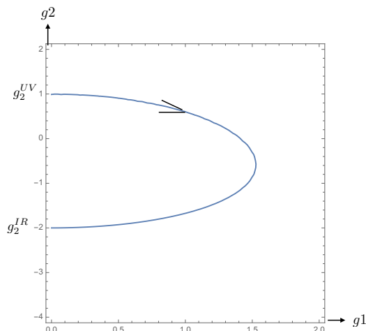
Figure 1. Massless flow in the imaginary sine-Gordon model from g_2^{UV} = 1 to g_2^{IR} = -2 . This corresponds to a flow from \beta_{UV} = \sqrt{3/5} to \beta_{IR} = \sqrt{3} . What is shown is a contour plot of the RG invariant \mathcal{I} .
