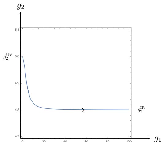
Figure 2. A massive flow in the imaginary sine-Gordon model from g_2^{\text{UV}} = 5 to g_2^{\text{IR}} = 24/5 . This corresponds to a flow from b_{\text{UV}} = 1/3 to b_{\text{IR}} = 1/\sqrt{11} . What is shown is a contour plot of the RG invariant \mathcal{I} where the x, y axes corresponds to g_1, g_2 .
