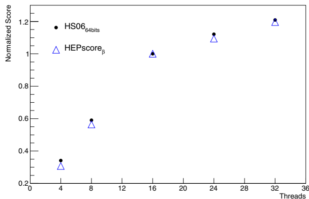
Fig. 10 \text{HS06}_{64\text{bits}} (points) and \text{HEPscore}_\beta (open triangles) measurements on the reference server when only a subset of the hardware threads were loaded by the benchmark application. The values have been normalized to the measurement using 16 threads, which corresponds to the number of physical cores of the server
