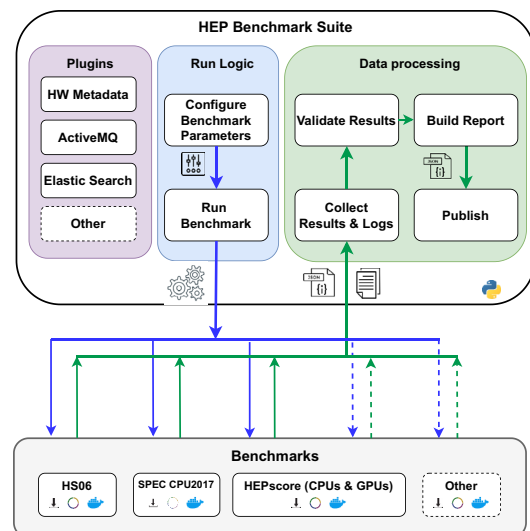
Fig. 4 HEP Benchmark Suite design. The figure depicts the Suite main functional blocks together with the decoupled benchmarks
