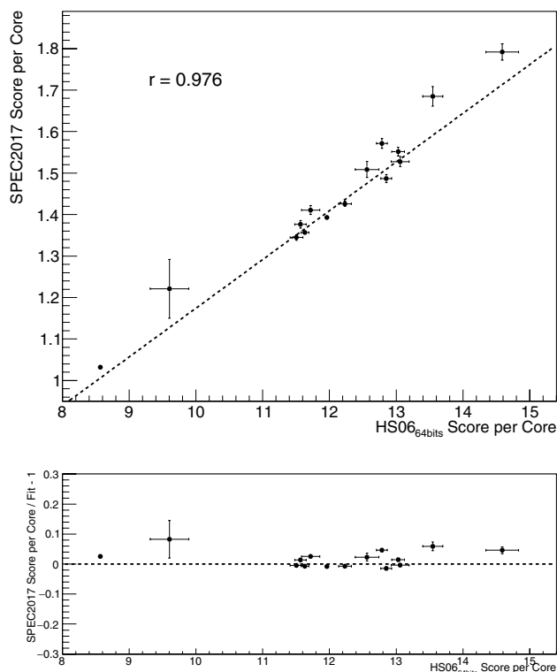
Fig. 1 SPEC CPU 2017 vs HS06 64bits scores (top). Each point corresponds to a different CPU model. The scores are normalized to the number of available cores. The correlation coefficient of the two samples is 0.976. The line is a linear fit to the data points where the y-intercept was fixed to zero. The normalized residuals with respect to the fit values are also reported (bottom). The data used in this plot were obtained from Ref. [7]
