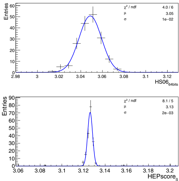
Fig. 9 Distribution of \text{HS06}_{64\text{bits}} (top) and \text{HEPscore}_\beta (bottom) scores of 180 identical servers normalized to the score of the reference server
