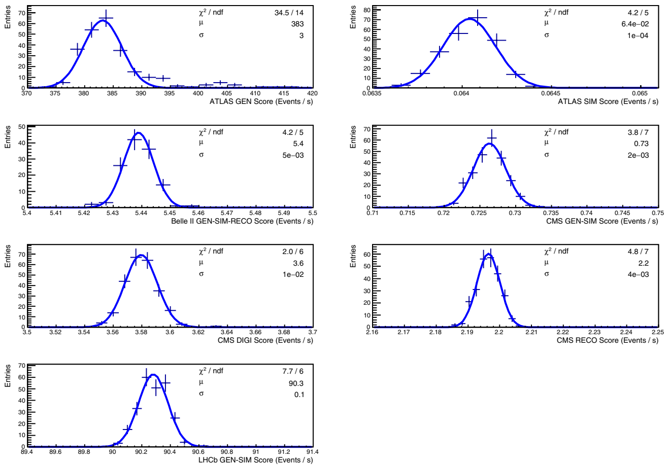
Fig. 3 Histograms of the measurements of the events processed per second of the seven HEP-Workloads on the reference server Intel(R) Xeon(R) CPU E5-2630 v3 @ 2.40 GHz, with hyper-threading ena-
