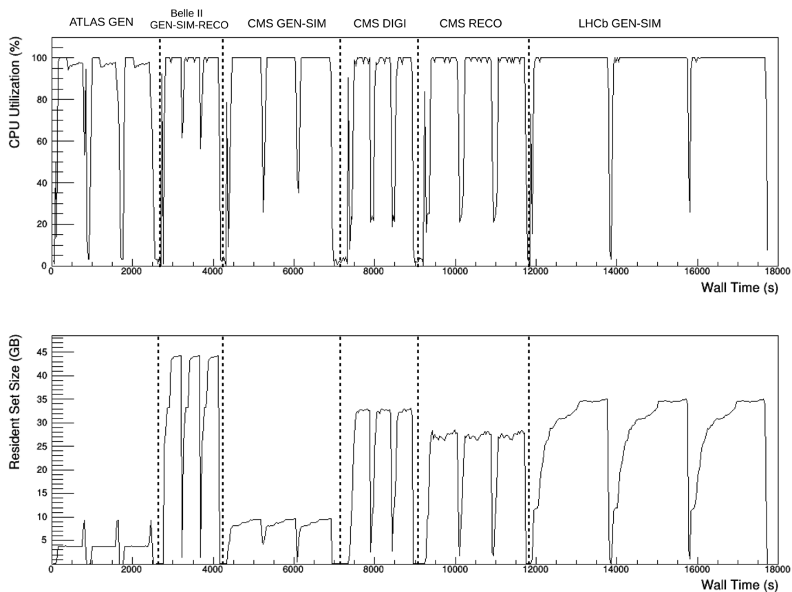
Fig. 7 CPU (top) and memory (bottom) utilization on the reference server measured during an \text{HEPscore}_\beta execution. The results show six different regions corresponding to the benchmark applications.
