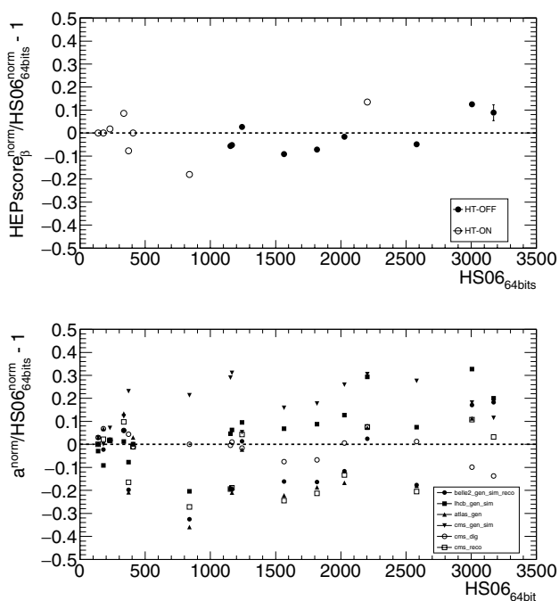
Fig. 8 Relative deviation of the \text{HEPscore}_\beta and \text{HS06}_{64\text{bits}} scores measured on multiple servers and normalized to the score of the reference server (top). Each CPU model is identified on the x-axis by the measured \text{HS06}_{64\text{bits}} score. The normalized score deviations from \text{HS06}_{64\text{bits}} for each application composing \text{HEPscore}_\beta are also reported (bottom). Each marker represents a given CPU model, with HT enabled (open circles) or disabled (full circles)
